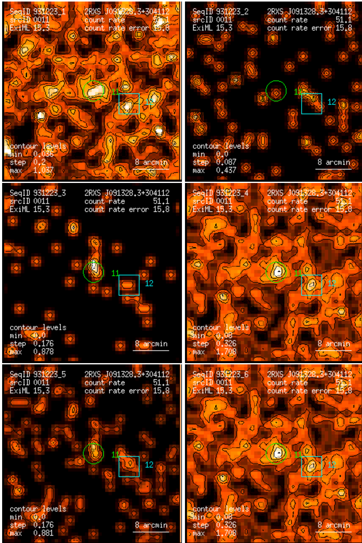
Figure 11: RASS 931223: detection 0011: band rate images, Gaussian filter: (1) PSPC channels 11 – 41, (2) 52 – 90, (3) 91 – 201, (4) 11 – 235, (5) 52 – 201, (6) 11 – 201. Broad band rates in counts/ks. Band rate contour levels in counts/ks/arcmin 2 .
