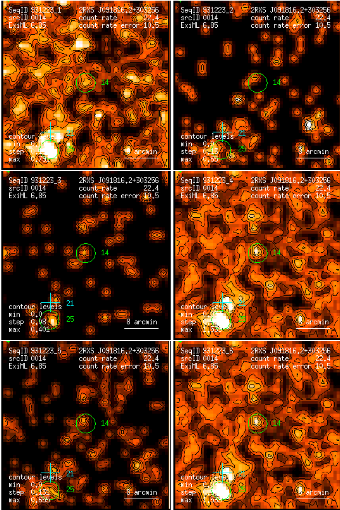
Figure 14: RASS 931223: detection 0014: band rate images, Gaussian filter: (1) PSPC channels 11 – 41, (2) 52 – 90, (3) 91 – 201, (4) 11 – 235, (5) 52 – 201, (6) 11 – 201. Broad band rates in counts/ks. Band rate contour levels in counts/ks/arcmin 2 .
