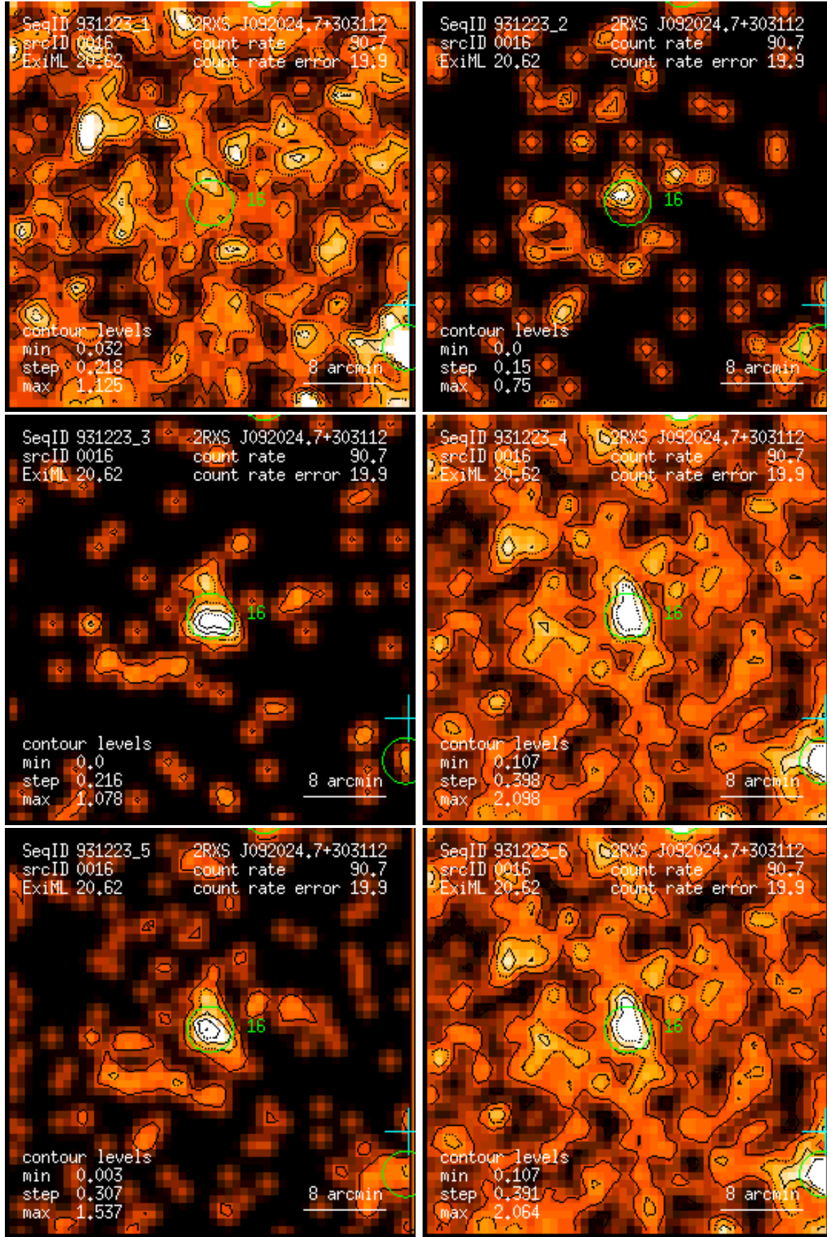
Figure 16: RASS 931223: detection 0016: band rate images, Gaussian filter: (1) PSPC channels 11 – 41, (2) 52 – 90, (3) 91 – 201, (4) 11 – 235, (5) 52 – 201, (6) 11 – 201. Broad band rates in counts/ks. Band rate contour levels in counts/ks/arcmin 2 .
