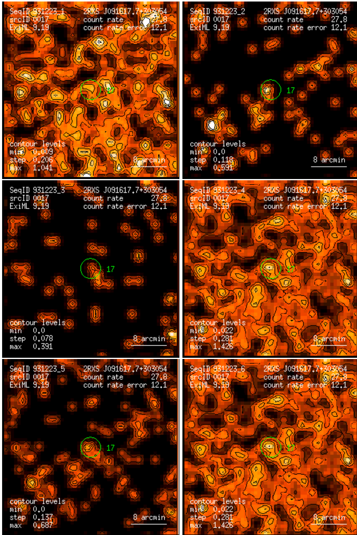
Figure 17: RASS 931223: detection 0017: band rate images, Gaussian filter: (1) PSPC channels 11 – 41, (2) 52 – 90, (3) 91 – 201, (4) 11 – 235, (5) 52 – 201, (6) 11 – 201. Broad band rates in counts/ks. Band rate contour levels in counts/ks/arcmin 2 .
