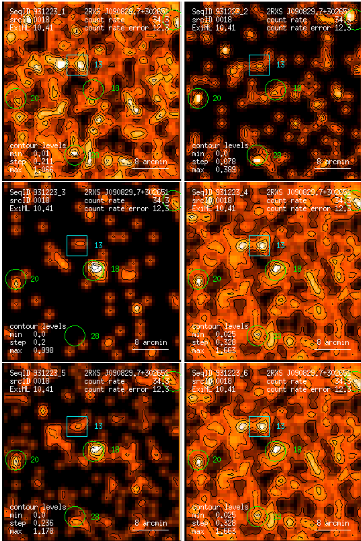
Figure 18: RASS 931223: detection 0018: band rate images, Gaussian filter: (1) PSPC channels 11 – 41, (2) 52 – 90, (3) 91 – 201, (4) 11 – 235, (5) 52 – 201, (6) 11 – 201. Broad band rates in counts/ks. Band rate contour levels in counts/ks/arcmin 2 .
