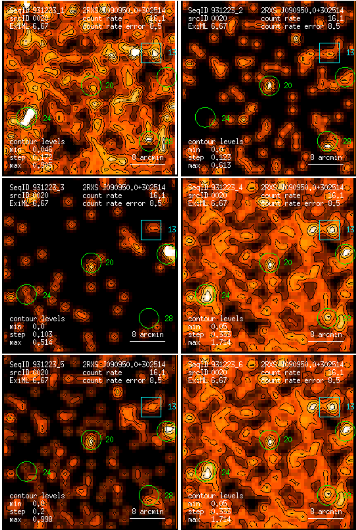
Figure 20: RASS 931223: detection 0020: band rate images, Gaussian filter: (1) PSPC channels 11 – 41, (2) 52 – 90, (3) 91 – 201, (4) 11 – 235, (5) 52 – 201, (6) 11 – 201. Broad band rates in counts/ks. Band rate contour levels in counts/ks/arcmin 2 .
