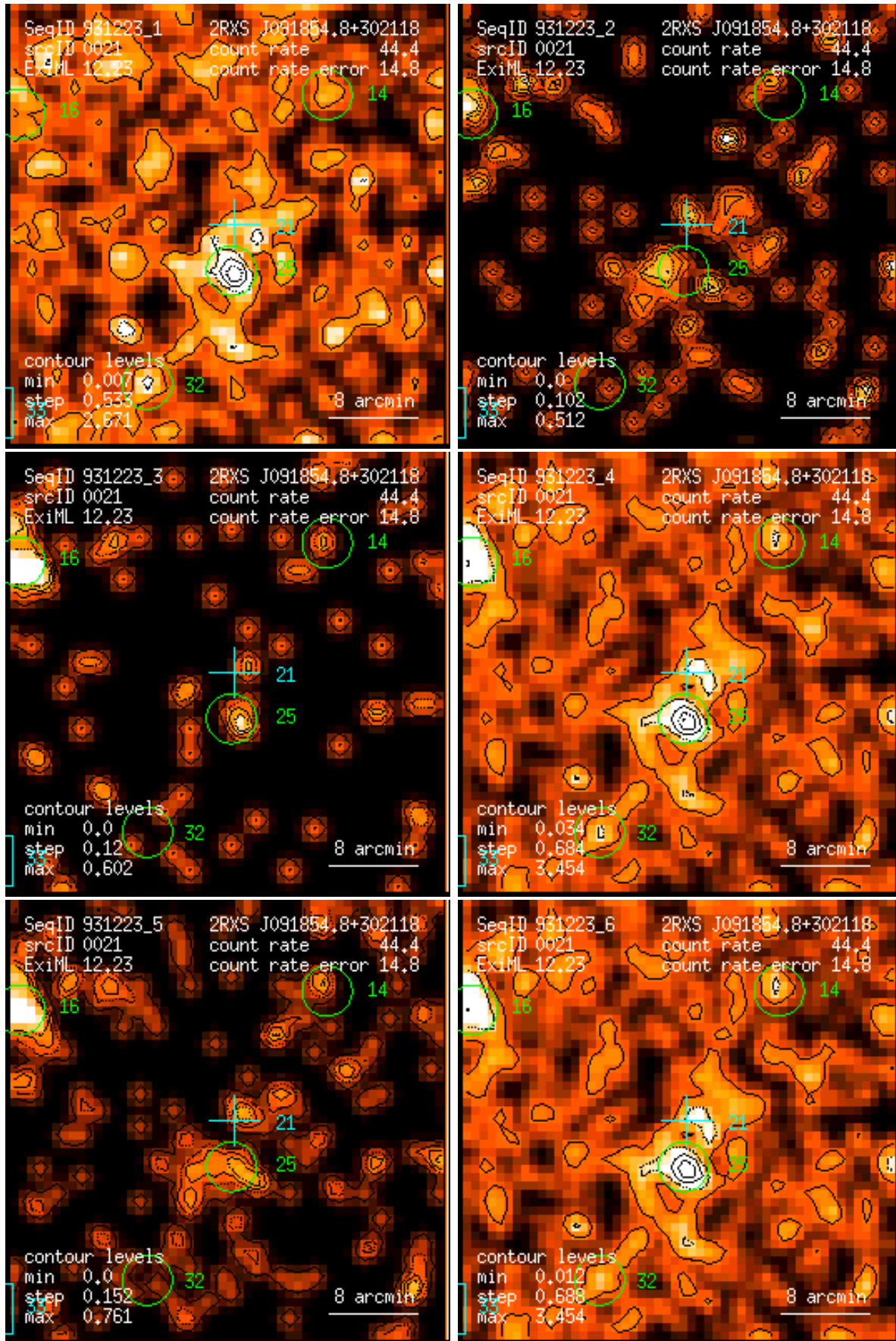
Figure 21: RASS 931223: detection 0021: band rate images, Gaussian filter: (1) PSPC channels 11 – 41, (2) 52 – 90, (3) 91 – 201, (4) 11 – 235, (5) 52 – 201, (6) 11 – 201. Broad band rates in counts/ks. Band rate contour levels in counts/ks/arcmin 2 .
