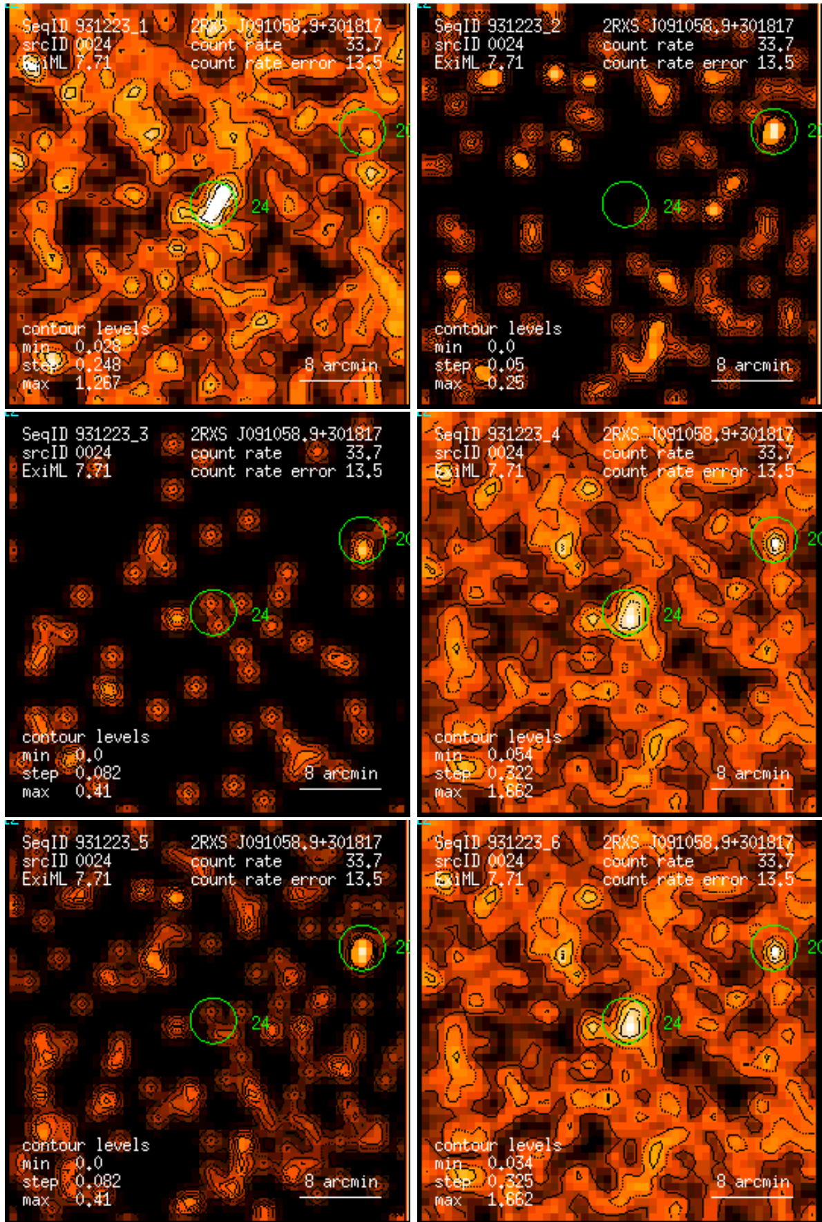
Figure 24: RASS 931223: detection 0024: band rate images, Gaussian filter: (1) PSPC channels 11 – 41, (2) 52 – 90, (3) 91 – 201, (4) 11 – 235, (5) 52 – 201, (6) 11 – 201. Broad band rates in counts/ks. Band rate contour levels in counts/ks/arcmin 2 .
