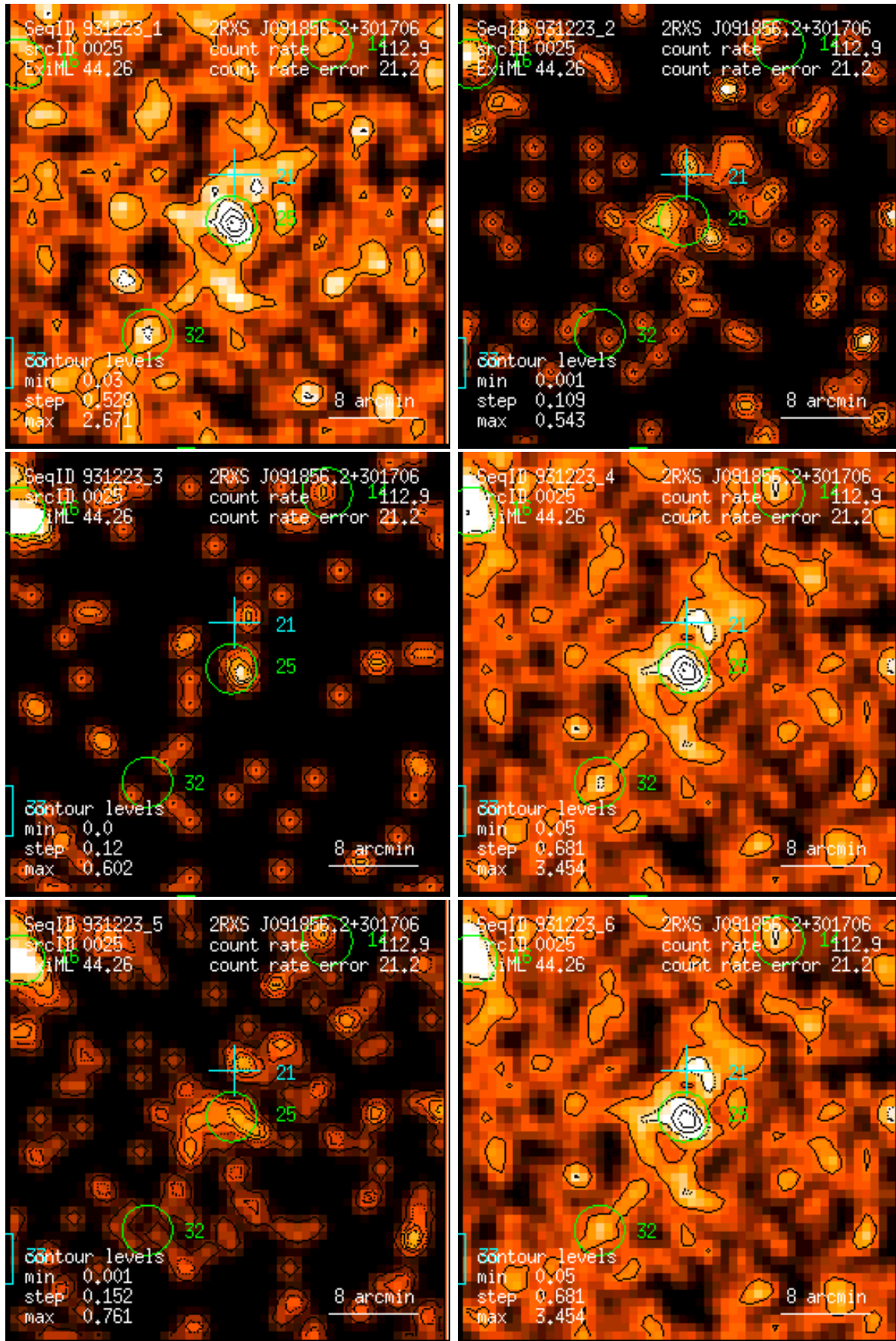
Figure 25: RASS 931223: detection 0025: band rate images, Gaussian filter: (1) PSPC channels 11 – 41, (2) 52 – 90, (3) 91 – 201, (4) 11 – 235, (5) 52 – 201, (6) 11 – 201. Broad band rates in counts/ks. Band rate contour levels in counts/ks/arcmin 2 .
