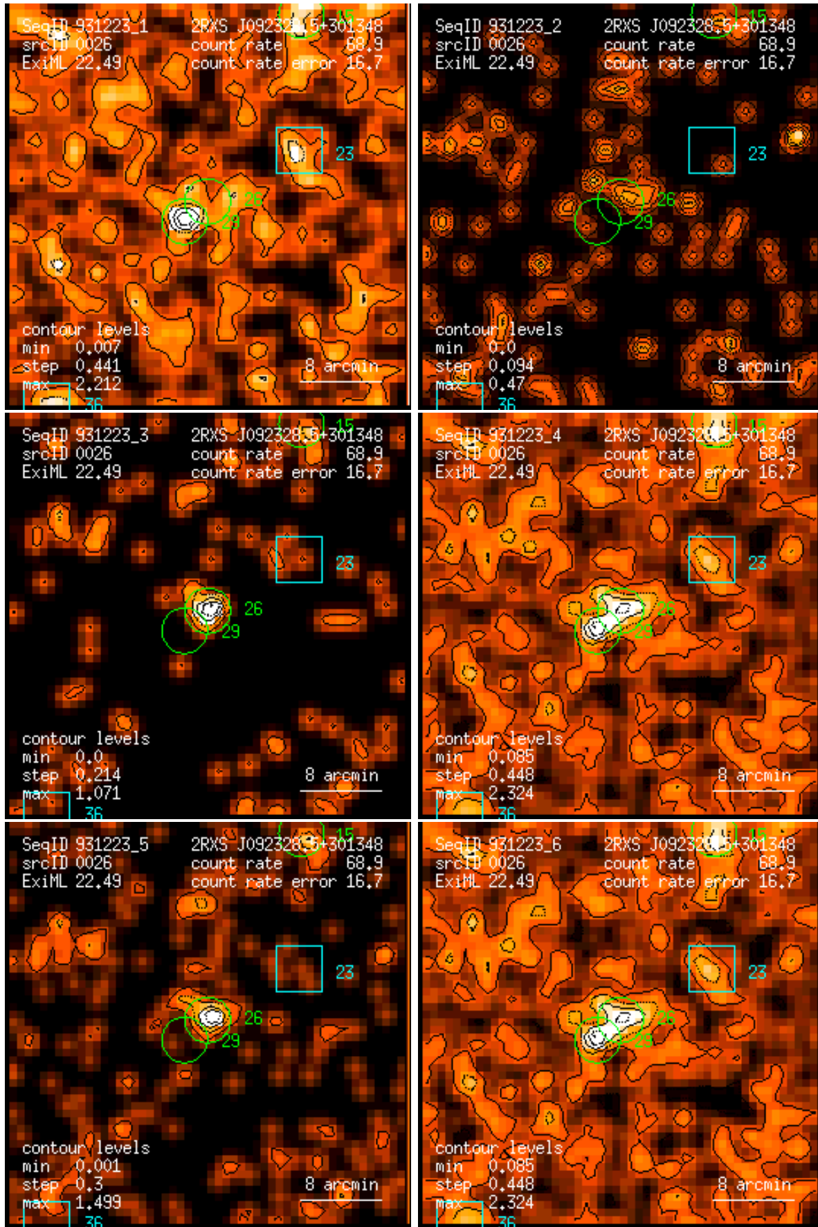
Figure 26: RASS 931223: detection 0026: band rate images, Gaussian filter: (1) PSPC channels 11 – 41, (2) 52 – 90, (3) 91 – 201, (4) 11 – 235, (5) 52 – 201, (6) 11 – 201. Broad band rates in counts/ks. Band rate contour levels in counts/ks/arcmin 2 .
