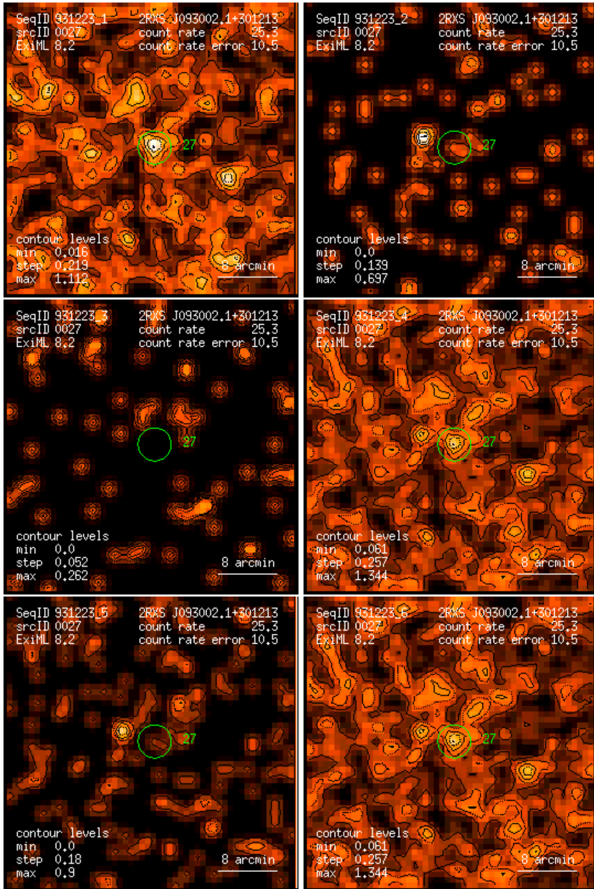
Figure 27: RASS 931223: detection 0027: band rate images, Gaussian filter: (1) PSPC channels 11 – 41, (2) 52 – 90, (3) 91 – 201, (4) 11 – 235, (5) 52 – 201, (6) 11 – 201. Broad band rates in counts/ks. Band rate contour levels in counts/ks/arcmin 2 .
