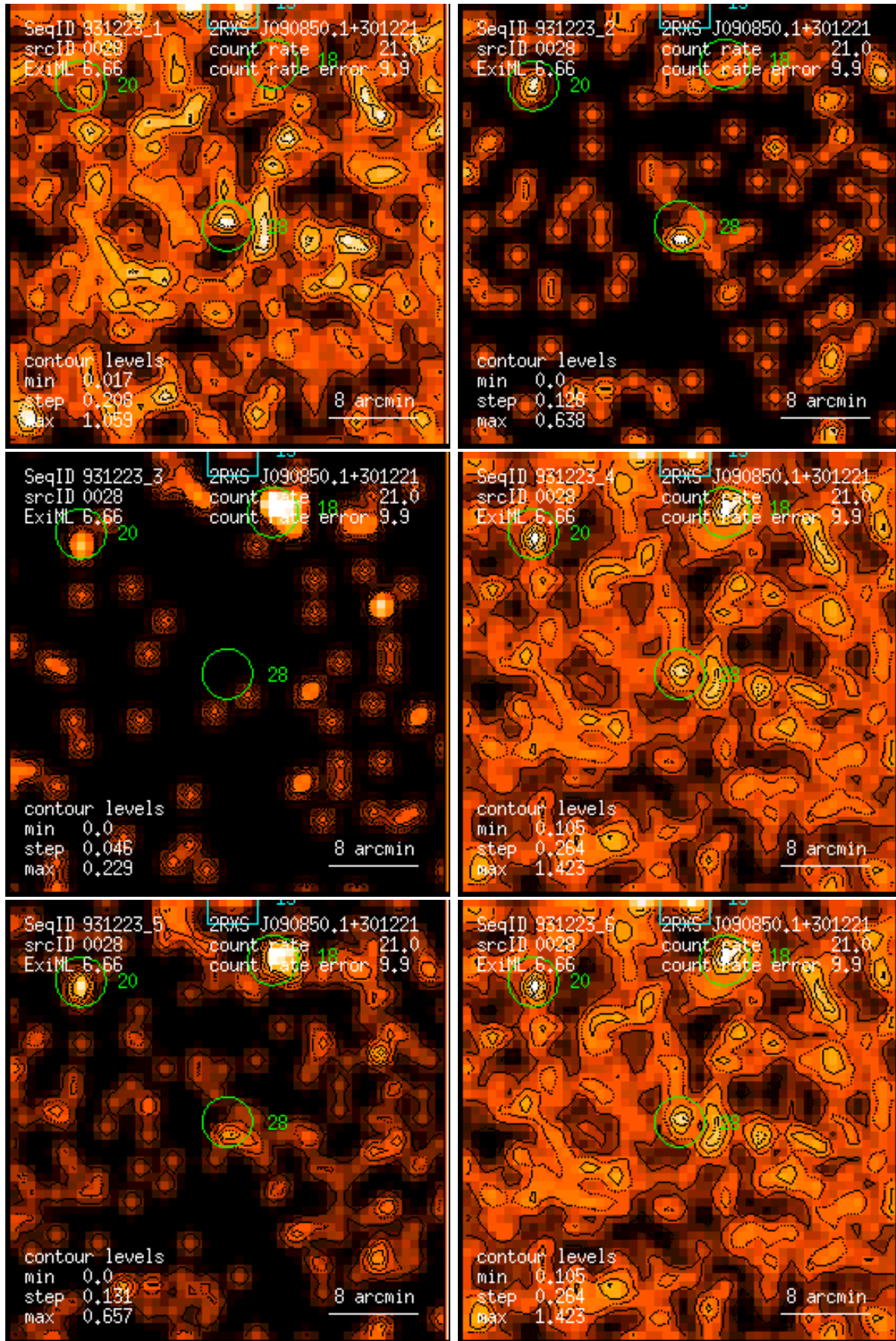
Figure 28: RASS 931223: detection 0028: band rate images, Gaussian filter: (1) PSPC channels 11 – 41, (2) 52 – 90, (3) 91 – 201, (4) 11 – 235, (5) 52 – 201, (6) 11 – 201. Broad band rates in counts/ks. Band rate contour levels in counts/ks/arcmin 2 .
