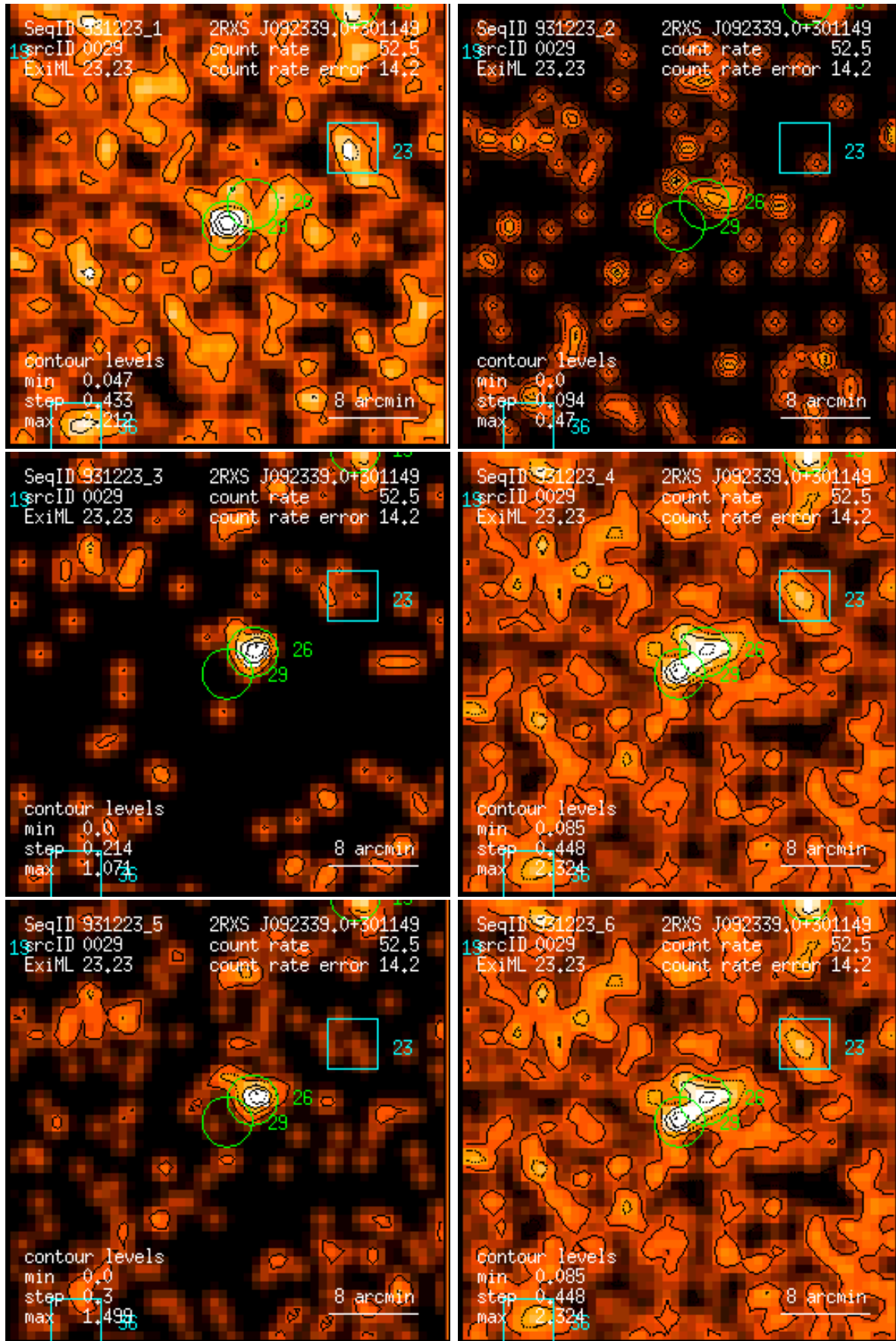
Figure 29: RASS 931223: detection 0029: band rate images, Gaussian filter: (1) PSPC channels 11 – 41, (2) 52 – 90, (3) 91 – 201, (4) 11 – 235, (5) 52 – 201, (6) 11 – 201. Broad band rates in counts/ks. Band rate contour levels in counts/ks/arcmin 2 .
