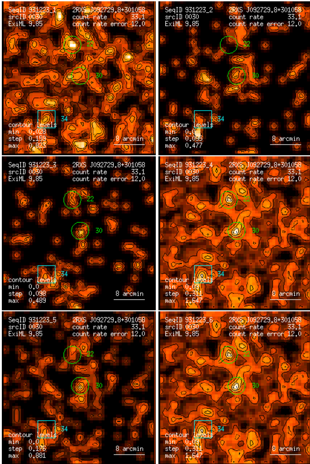
Figure 30: RASS 931223: detection 0030: band rate images, Gaussian filter: (1) PSPC channels 11 – 41, (2) 52 – 90, (3) 91 – 201, (4) 11 – 235, (5) 52 – 201, (6) 11 – 201. Broad band rates in counts/ks. Band rate contour levels in counts/ks/arcmin 2 .
