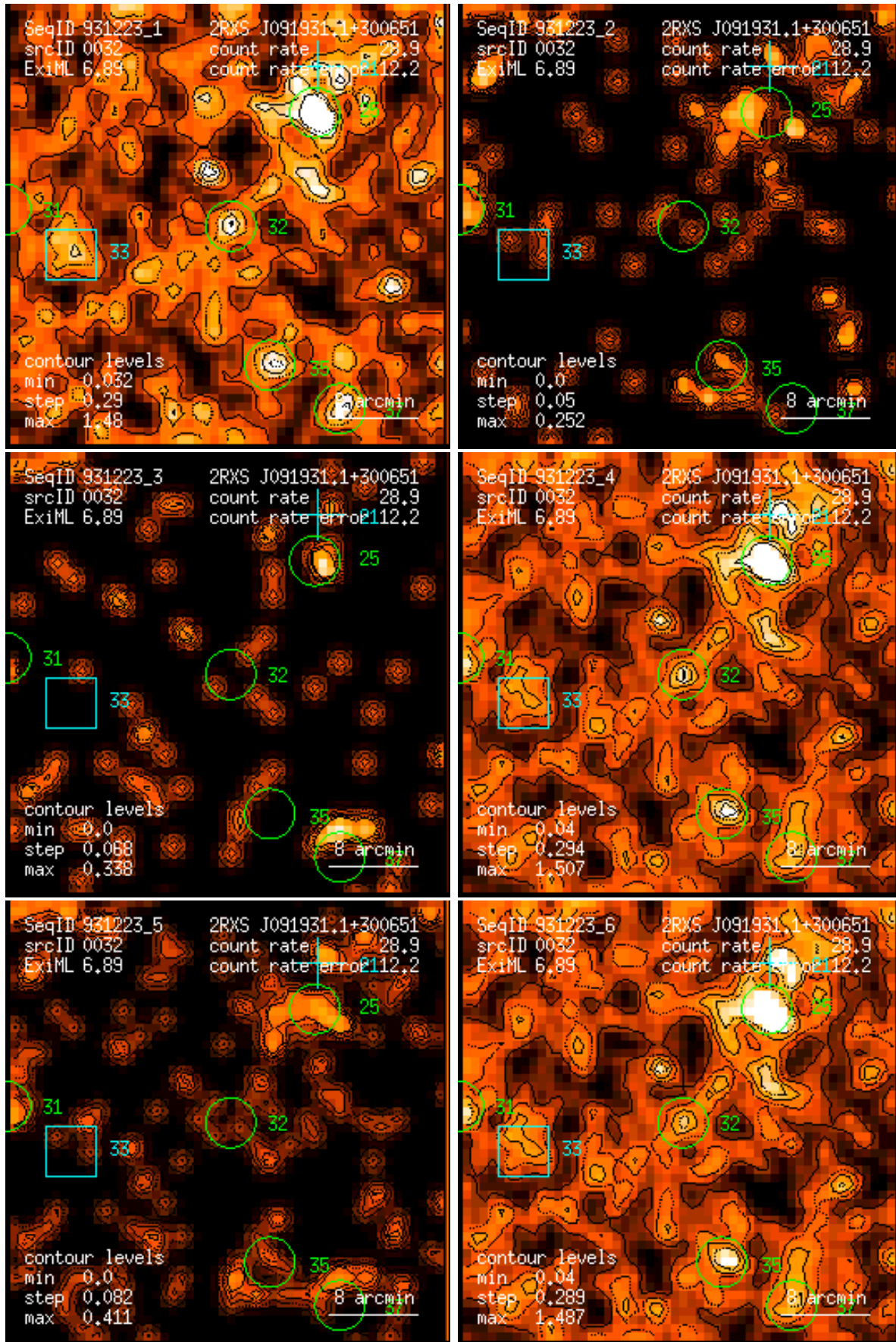
Figure 32: RASS 931223: detection 0032: band rate images, Gaussian filter: (1) PSPC channels 11 – 41, (2) 52 – 90, (3) 91 – 201, (4) 11 – 235, (5) 52 – 201, (6) 11 – 201. Broad band rates in counts/ks. Band rate contour levels in counts/ks/arcmin 2 .
