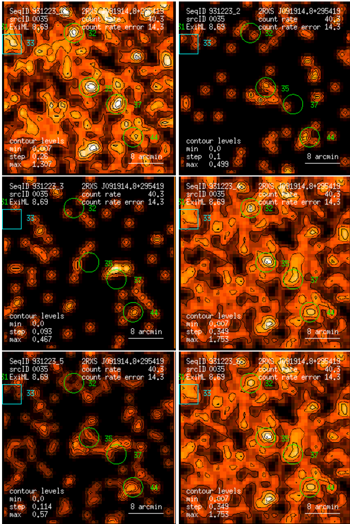
Figure 35: RASS 931223: detection 0035: band rate images, Gaussian filter: (1) PSPC channels 11 – 41, (2) 52 – 90, (3) 91 – 201, (4) 11 – 235, (5) 52 – 201, (6) 11 – 201. Broad band rates in counts/ks. Band rate contour levels in counts/ks/arcmin 2 .
