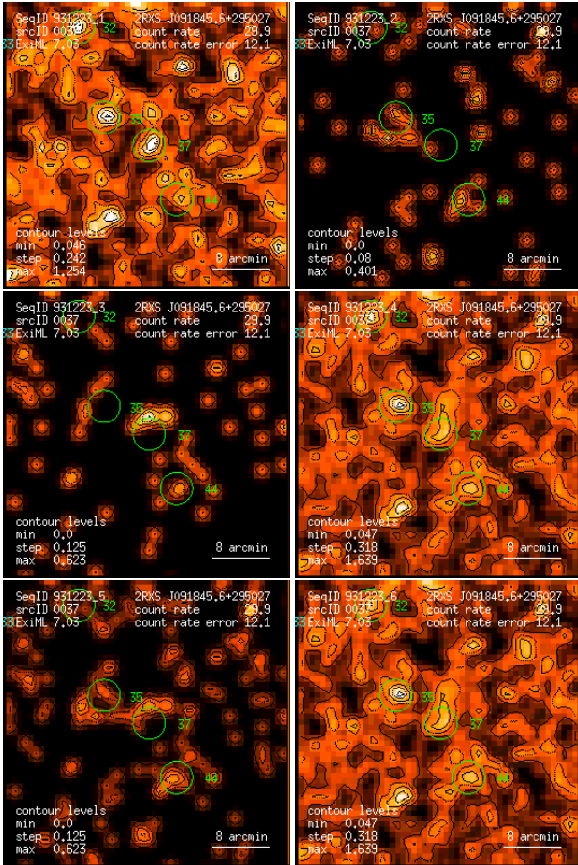
Figure 37: RASS 931223: detection 0037: band rate images, Gaussian filter: (1) PSPC channels 11 – 41, (2) 52 – 90, (3) 91 – 201, (4) 11 – 235, (5) 52 – 201, (6) 11 – 201. Broad band rates in counts/ks. Band rate contour levels in counts/ks/arcmin 2 .
