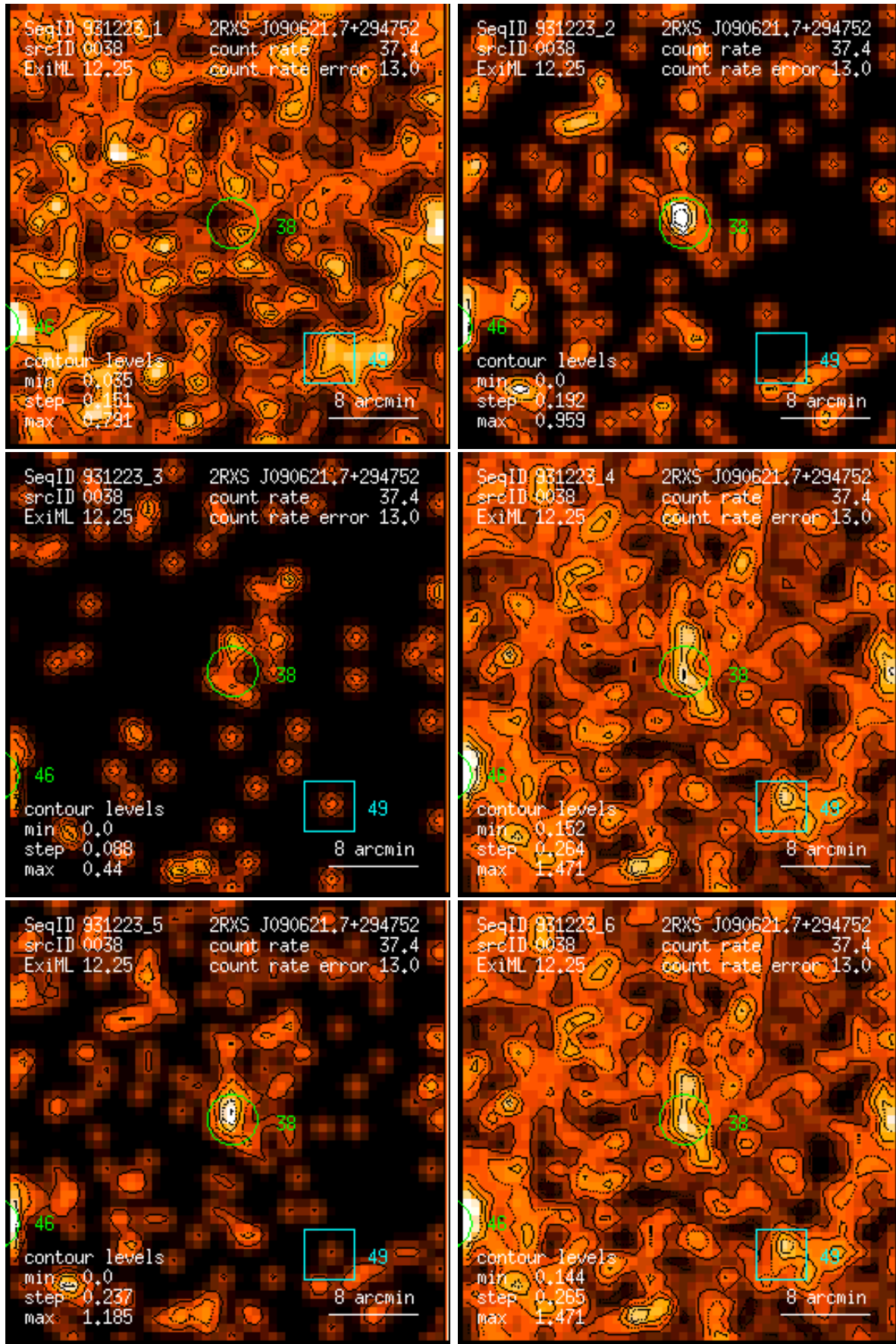
Figure 38: RASS 931223: detection 0038: band rate images, Gaussian filter: (1) PSPC channels 11 – 41, (2) 52 – 90, (3) 91 – 201, (4) 11 – 235, (5) 52 – 201, (6) 11 – 201. Broad band rates in counts/ks. Band rate contour levels in counts/ks/arcmin 2 .
