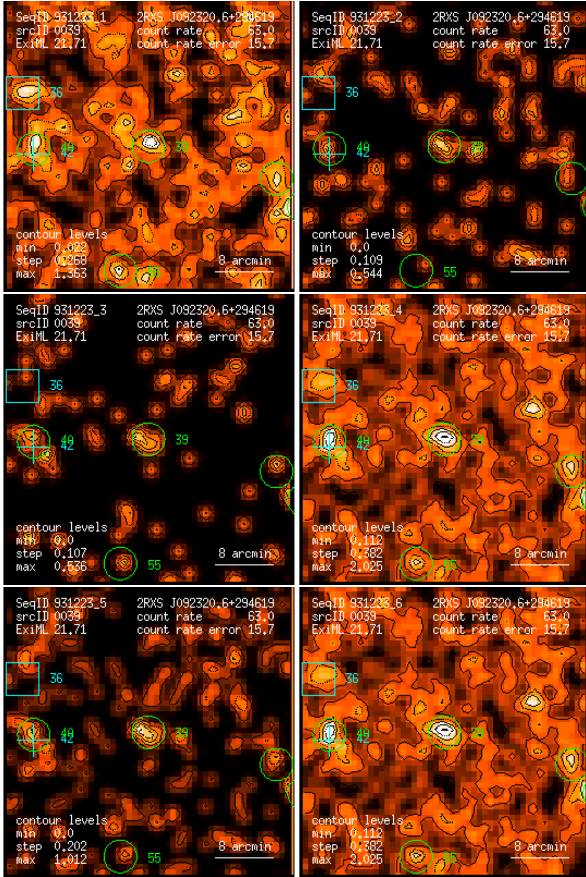
Figure 39: RASS 931223: detection 0039: band rate images, Gaussian filter: (1) PSPC channels 11 – 41, (2) 52 – 90, (3) 91 – 201, (4) 11 – 235, (5) 52 – 201, (6) 11 – 201. Broad band rates in counts/ks. Band rate contour levels in counts/ks/arcmin 2 .
