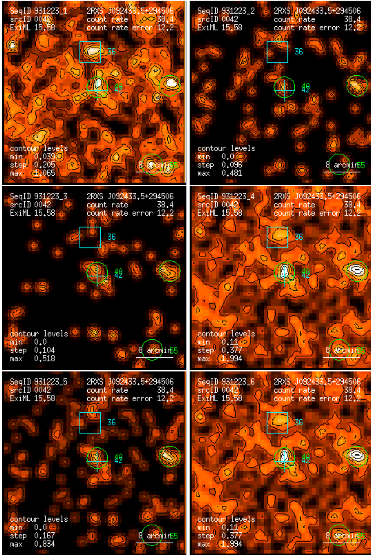
Figure 42: RASS 931223: detection 0042: band rate images, Gaussian filter: (1) PSPC channels 11 – 41, (2) 52 – 90, (3) 91 – 201, (4) 11 – 235, (5) 52 – 201, (6) 11 – 201. Broad band rates in counts/ks. Band rate contour levels in counts/ks/arcmin 2 .
