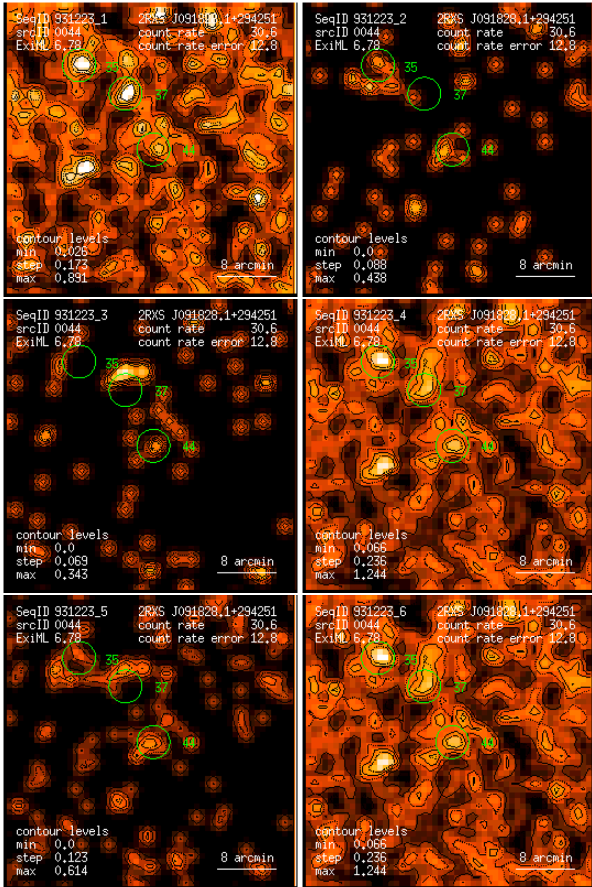
Figure 44: RASS 931223: detection 0044: band rate images, Gaussian filter: (1) PSPC channels 11 – 41, (2) 52 – 90, (3) 91 – 201, (4) 11 – 235, (5) 52 – 201, (6) 11 – 201. Broad band rates in counts/ks. Band rate contour levels in counts/ks/arcmin 2 .
