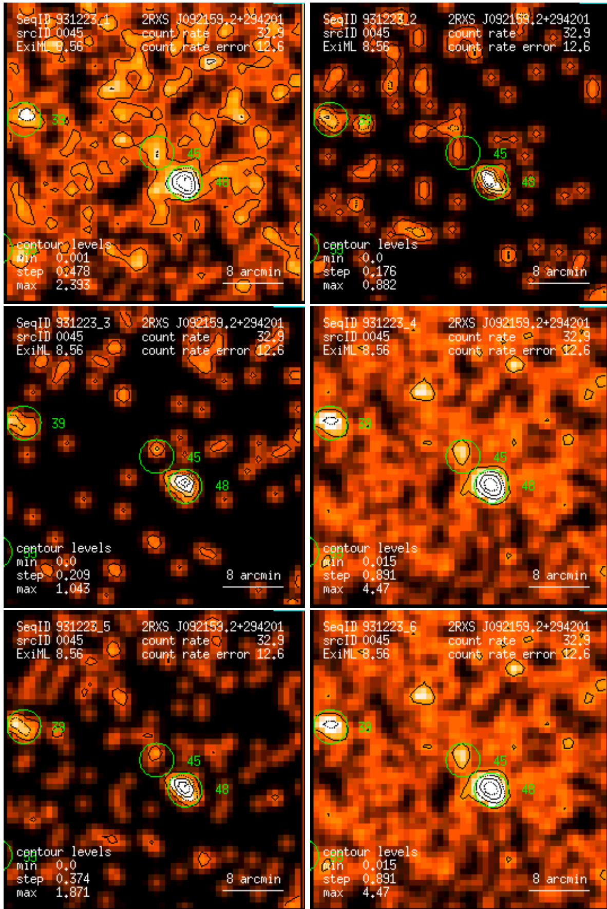
Figure 45: RASS 931223: detection 0045: band rate images, Gaussian filter: (1) PSPC channels 11 – 41, (2) 52 – 90, (3) 91 – 201, (4) 11 – 235, (5) 52 – 201, (6) 11 – 201. Broad band rates in counts/ks. Band rate contour levels in counts/ks/arcmin 2 .
