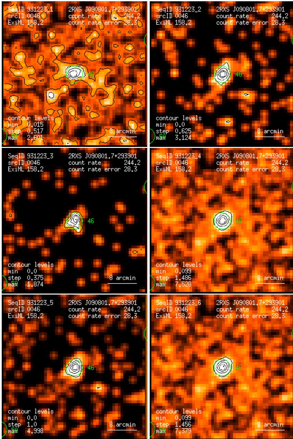
Figure 46: RASS 931223: detection 0046: band rate images, Gaussian filter: (1) PSPC channels 11 – 41, (2) 52 – 90, (3) 91 – 201, (4) 11 – 235, (5) 52 – 201, (6) 11 – 201. Broad band rates in counts/ks. Band rate contour levels in counts/ks/arcmin 2 .
