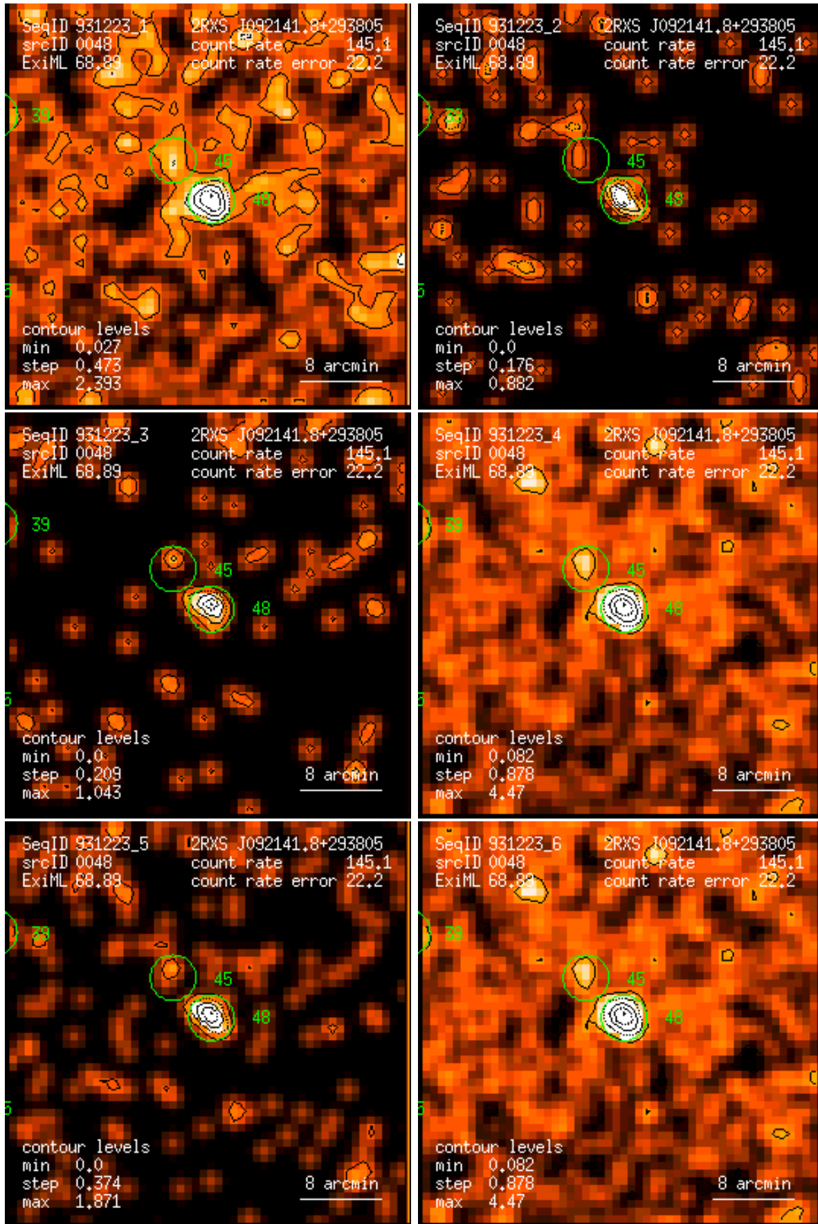
Figure 48: RASS 931223: detection 0048: band rate images, Gaussian filter: (1) PSPC channels 11 – 41, (2) 52 – 90, (3) 91 – 201, (4) 11 – 235, (5) 52 – 201, (6) 11 – 201. Broad band rates in counts/ks. Band rate contour levels in counts/ks/arcmin 2 .
