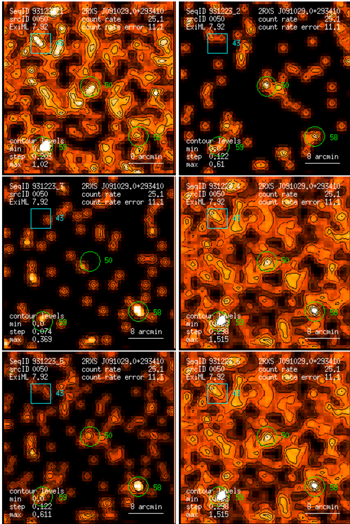
Figure 50: RASS 931223: detection 0050: band rate images, Gaussian filter: (1) PSPC channels 11 – 41, (2) 52 – 90, (3) 91 – 201, (4) 11 – 235, (5) 52 – 201, (6) 11 – 201. Broad band rates in counts/ks. Band rate contour levels in counts/ks/arcmin 2 .
