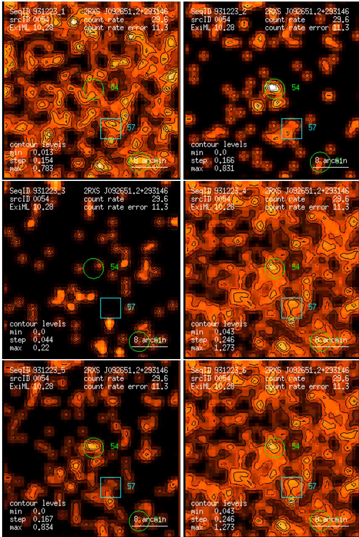
Figure 54: RASS 931223: detection 0054: band rate images, Gaussian filter: (1) PSPC channels 11 – 41, (2) 52 – 90, (3) 91 – 201, (4) 11 – 235, (5) 52 – 201, (6) 11 – 201. Broad band rates in counts/ks. Band rate contour levels in counts/ks/arcmin 2 .
