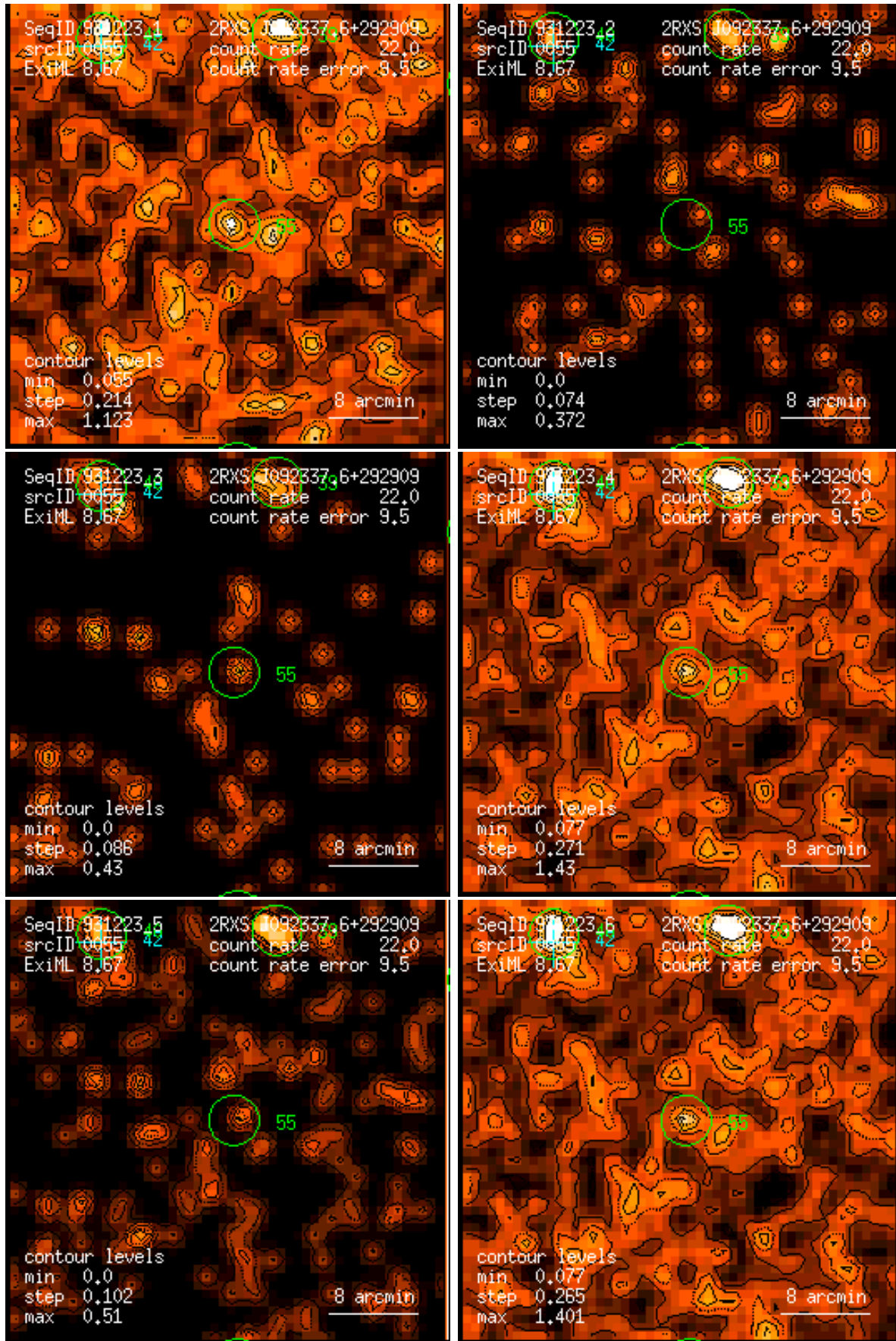
Figure 55: RASS 931223: detection 0055: band rate images, Gaussian filter: (1) PSPC channels 11 – 41, (2) 52 – 90, (3) 91 – 201, (4) 11 – 235, (5) 52 – 201, (6) 11 – 201. Broad band rates in counts/ks. Band rate contour levels in counts/ks/arcmin 2 .
