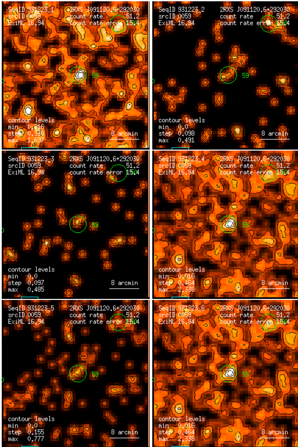
Figure 59: RASS 931223: detection 0059: band rate images, Gaussian filter: (1) PSPC channels 11 – 41, (2) 52 – 90, (3) 91 – 201, (4) 11 – 235, (5) 52 – 201, (6) 11 – 201. Broad band rates in counts/ks. Band rate contour levels in counts/ks/arcmin 2 .
