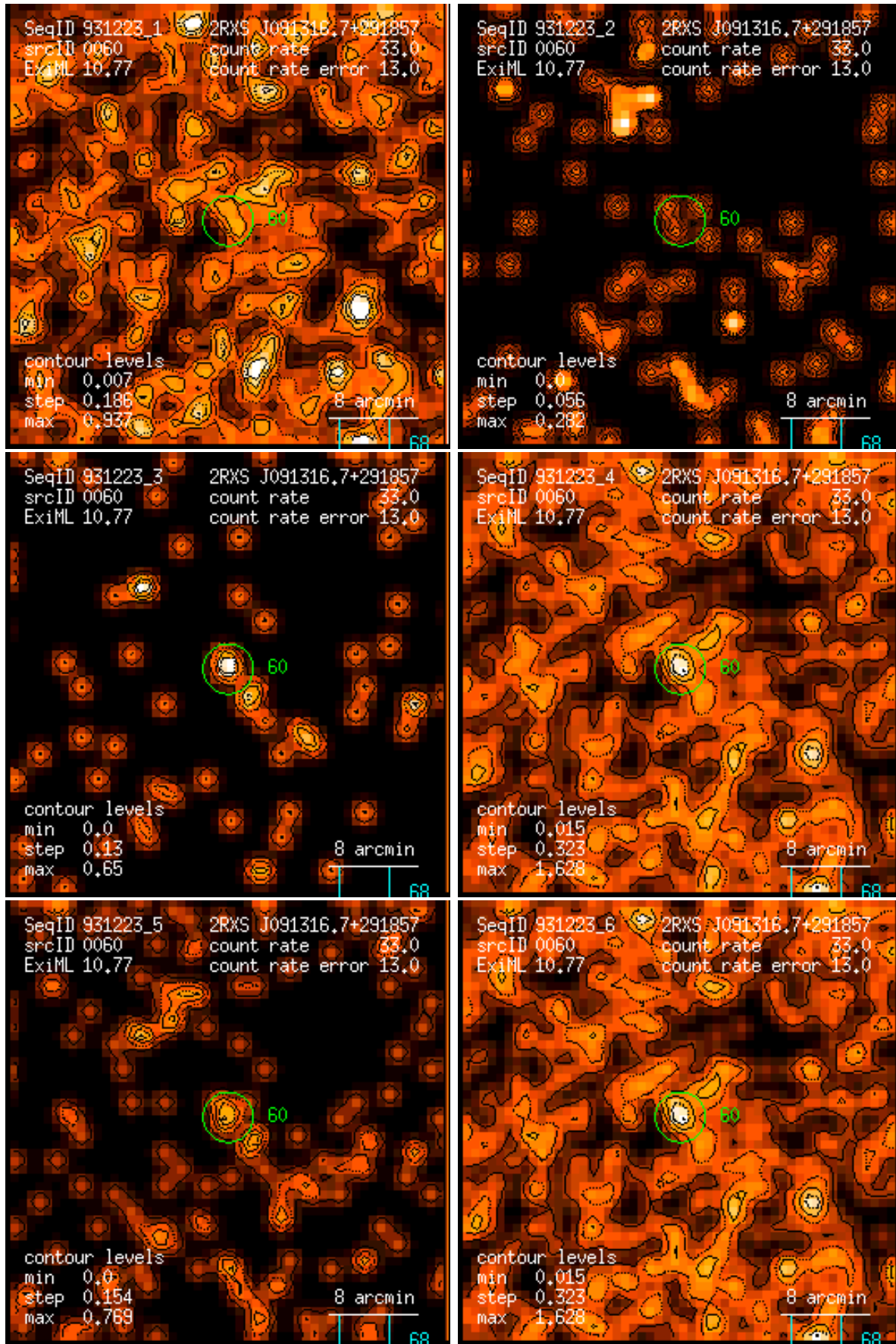
Figure 60: RASS 931223: detection 0060: band rate images, Gaussian filter: (1) PSPC channels 11 – 41, (2) 52 – 90, (3) 91 – 201, (4) 11 – 235, (5) 52 – 201, (6) 11 – 201. Broad band rates in counts/ks. Band rate contour levels in counts/ks/arcmin 2 .
