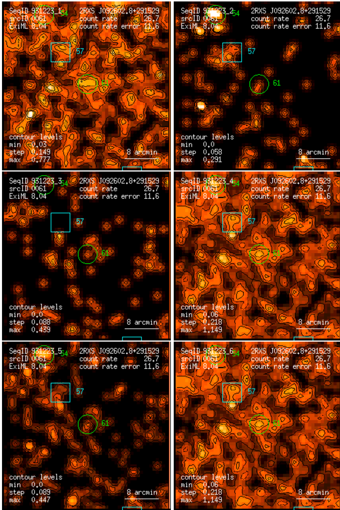
Figure 61: RASS 931223: detection 0061: band rate images, Gaussian filter: (1) PSPC channels 11 – 41, (2) 52 – 90, (3) 91 – 201, (4) 11 – 235, (5) 52 – 201, (6) 11 – 201. Broad band rates in counts/ks. Band rate contour levels in counts/ks/arcmin 2 .
