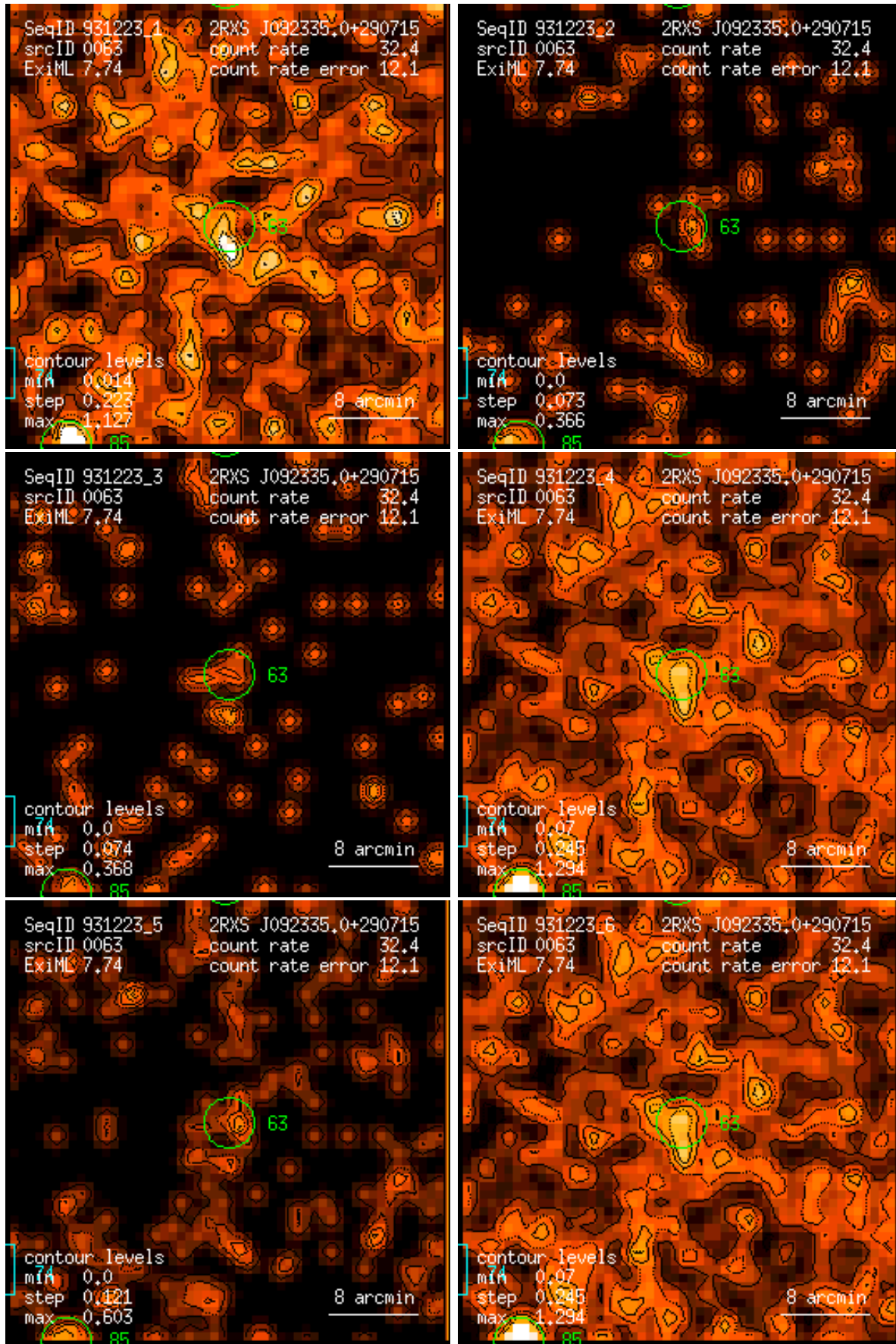
Figure 63: RASS 931223: detection 0063: band rate images, Gaussian filter: (1) PSPC channels 11 – 41, (2) 52 – 90, (3) 91 – 201, (4) 11 – 235, (5) 52 – 201, (6) 11 – 201. Broad band rates in counts/ks. Band rate contour levels in counts/ks/arcmin 2 .
