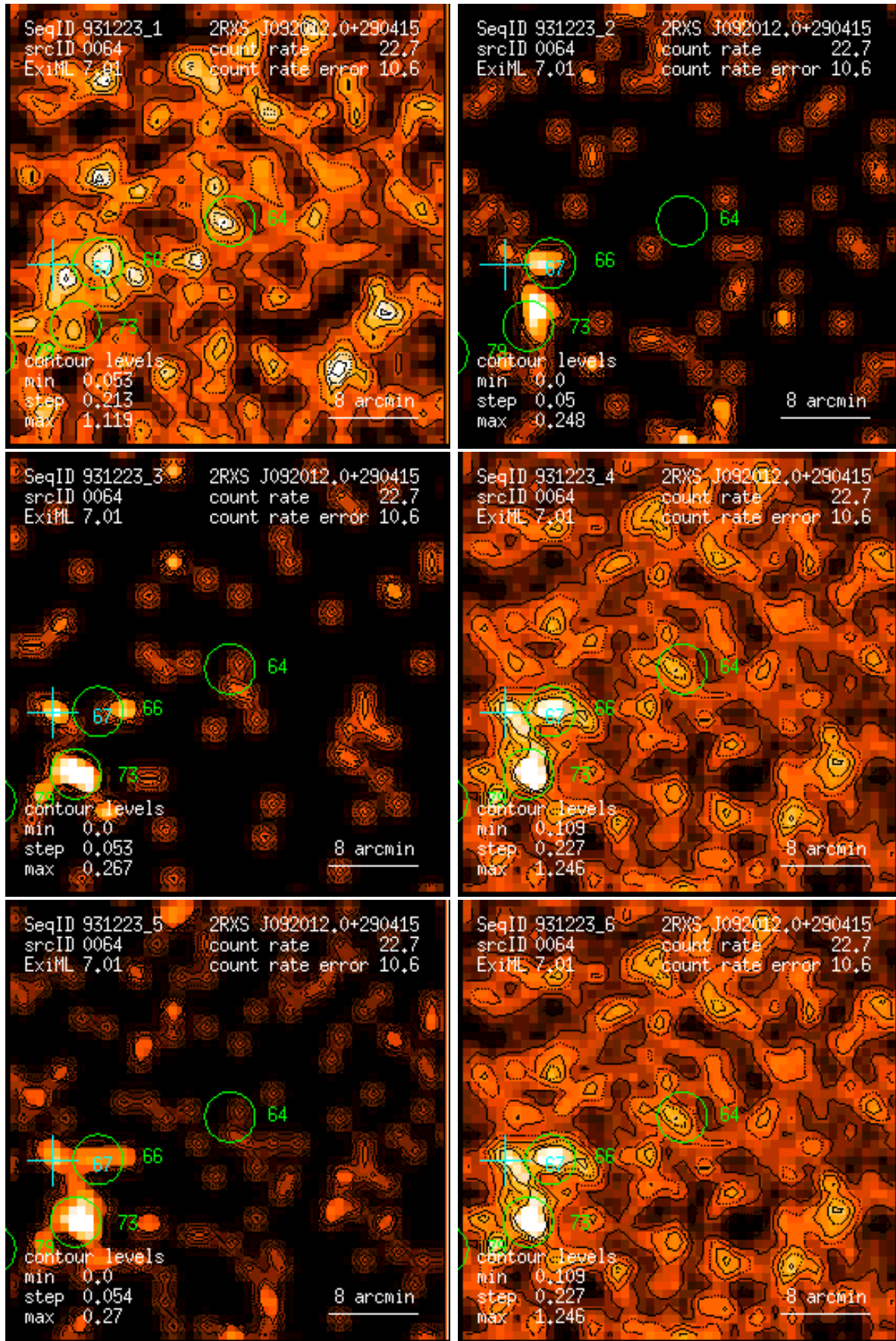
Figure 64: RASS 931223: detection 0064: band rate images, Gaussian filter: (1) PSPC channels 11 – 41, (2) 52 – 90, (3) 91 – 201, (4) 11 – 235, (5) 52 – 201, (6) 11 – 201. Broad band rates in counts/ks. Band rate contour levels in counts/ks/arcmin 2 .
