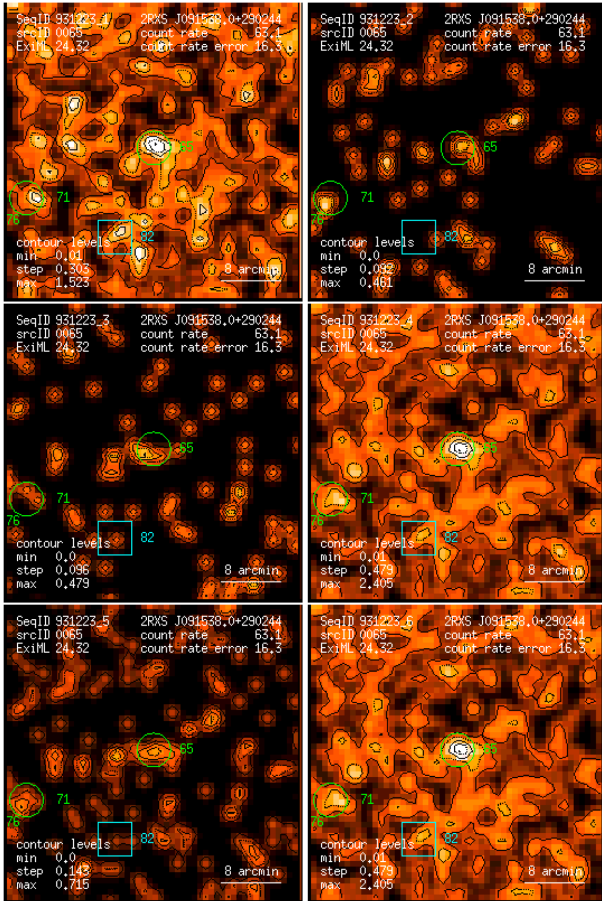
Figure 65: RASS 931223: detection 0065: band rate images, Gaussian filter: (1) PSPC channels 11 – 41, (2) 52 – 90, (3) 91 – 201, (4) 11 – 235, (5) 52 – 201, (6) 11 – 201. Broad band rates in counts/ks. Band rate contour levels in counts/ks/arcmin 2 .
