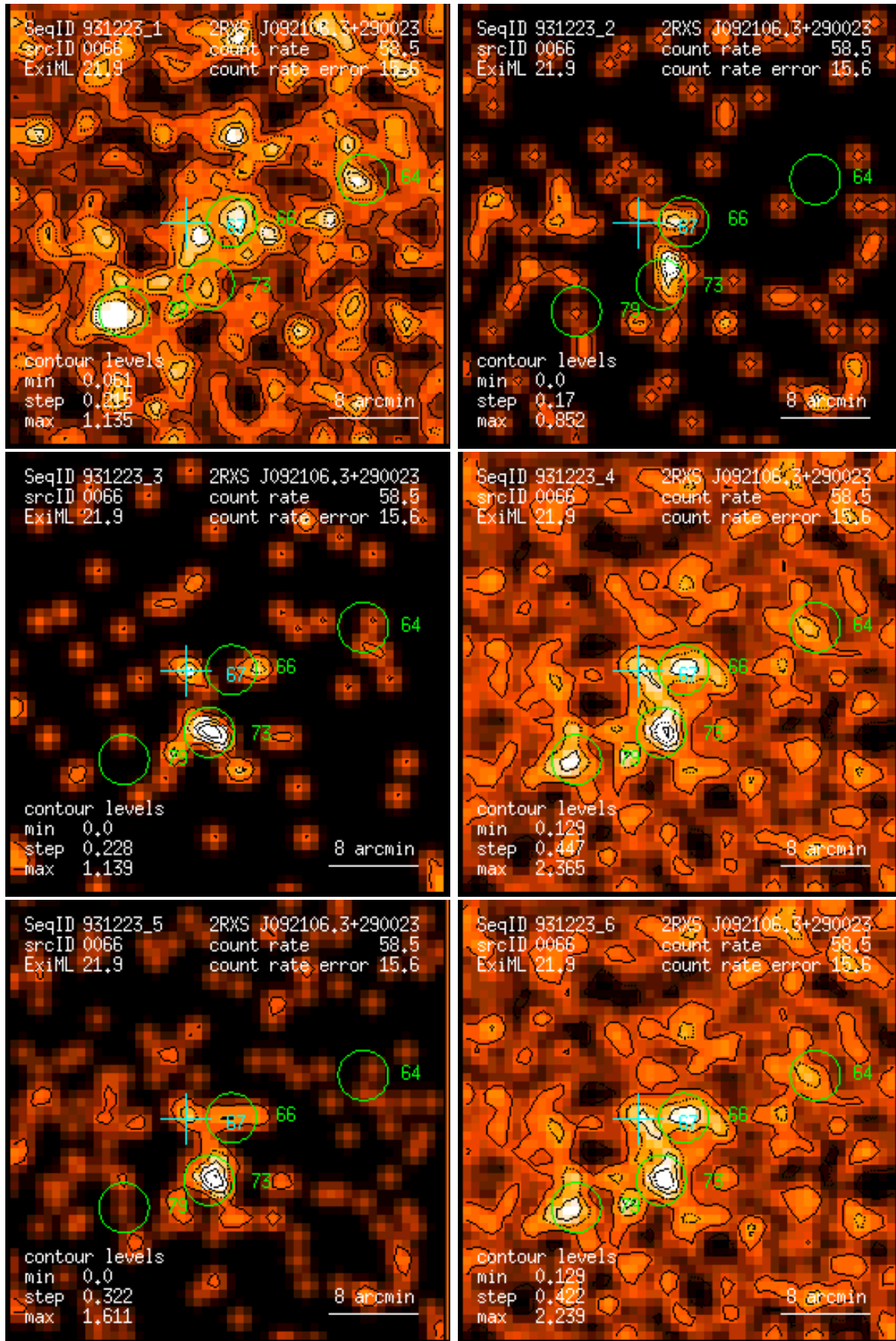
Figure 66: RASS 931223: detection 0066: band rate images, Gaussian filter: (1) PSPC channels 11 – 41, (2) 52 – 90, (3) 91 – 201, (4) 11 – 235, (5) 52 – 201, (6) 11 – 201. Broad band rates in counts/ks. Band rate contour levels in counts/ks/arcmin 2 .
