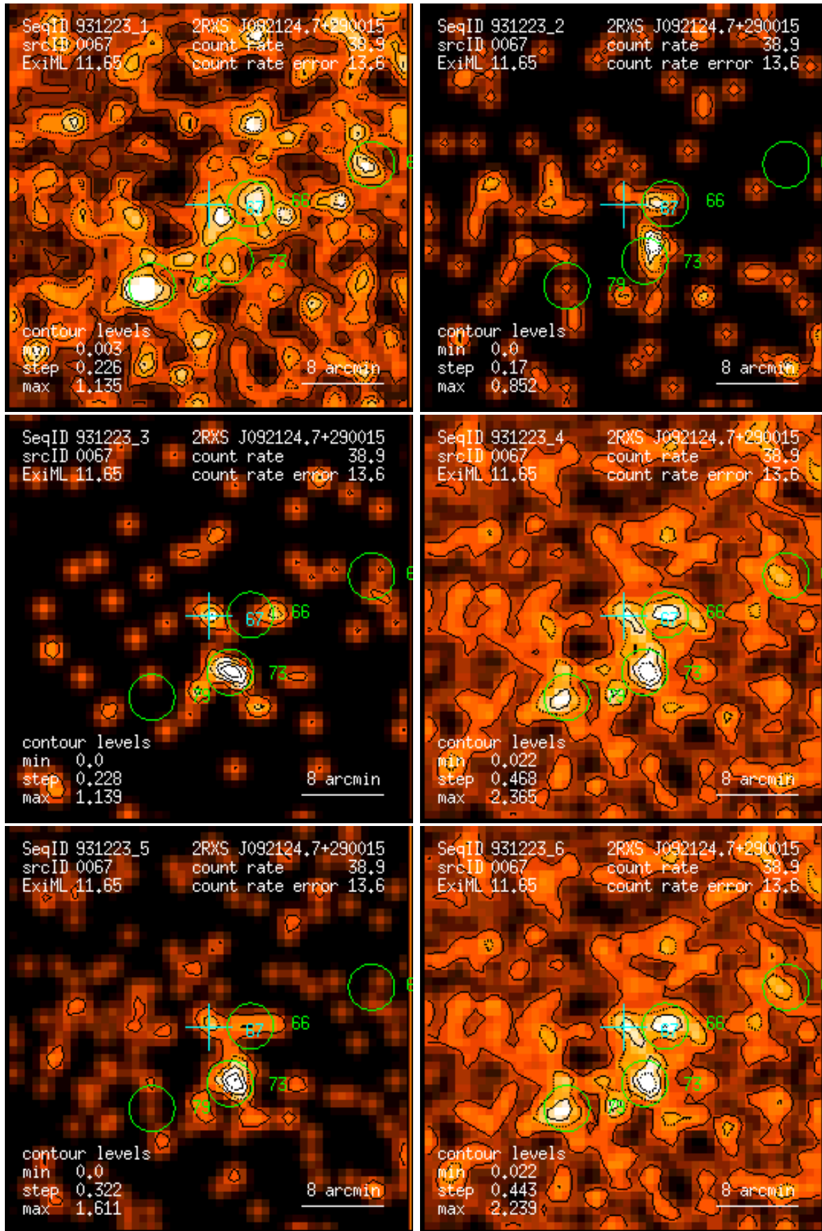
Figure 67: RASS 931223: detection 0067: band rate images, Gaussian filter: (1) PSPC channels 11 – 41, (2) 52 – 90, (3) 91 – 201, (4) 11 – 235, (5) 52 – 201, (6) 11 – 201. Broad band rates in counts/ks. Band rate contour levels in counts/ks/arcmin 2 .
