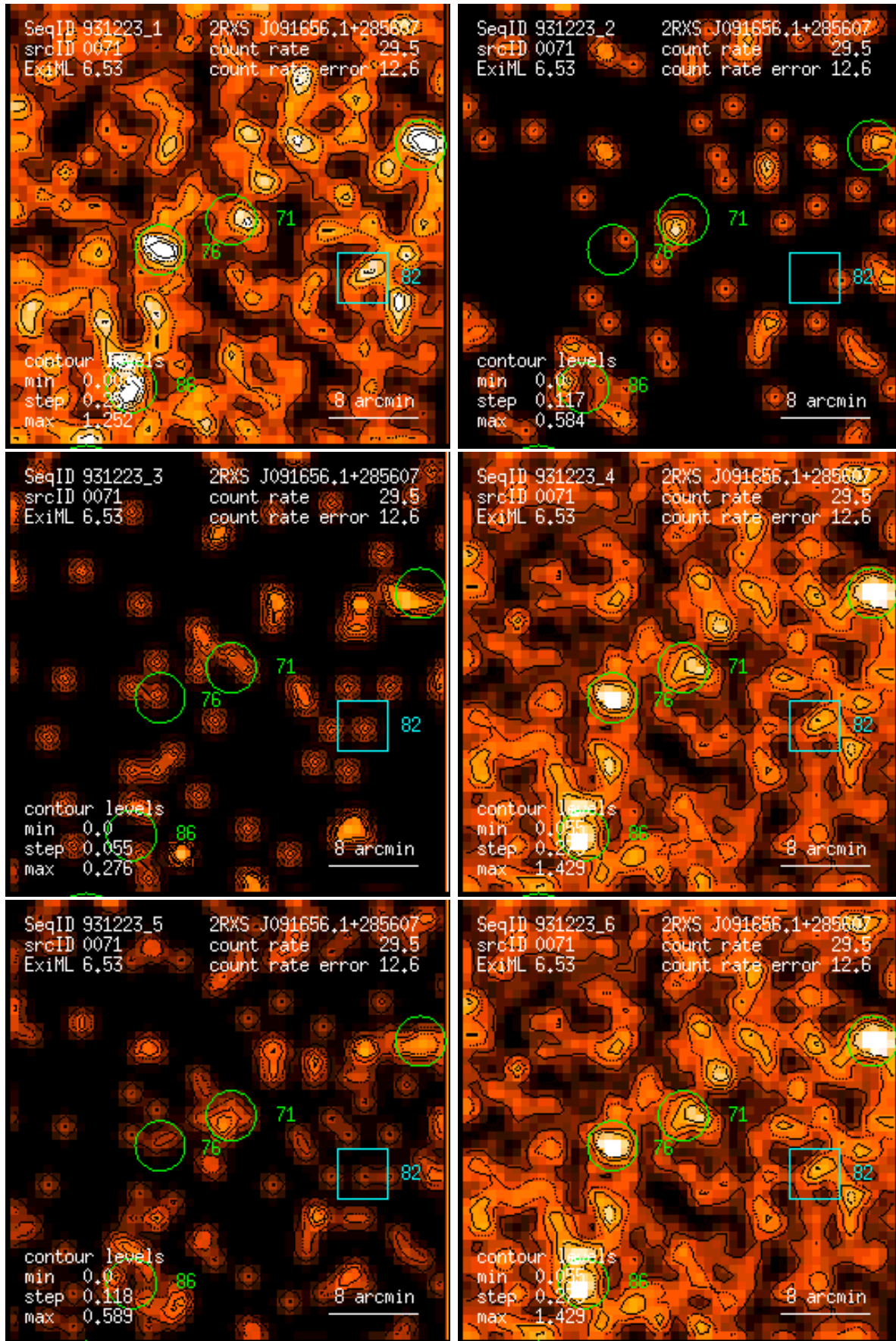
Figure 71: RASS 931223: detection 0071: band rate images, Gaussian filter: (1) PSPC channels 11 – 41, (2) 52 – 90, (3) 91 – 201, (4) 11 – 235, (5) 52 – 201, (6) 11 – 201. Broad band rates in counts/ks. Band rate contour levels in counts/ks/arcmin 2 .
