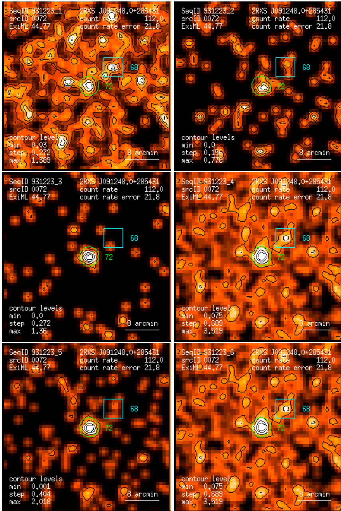
Figure 72: RASS 931223: detection 0072: band rate images, Gaussian filter: (1) PSPC channels 11 – 41, (2) 52 – 90, (3) 91 – 201, (4) 11 – 235, (5) 52 – 201, (6) 11 – 201. Broad band rates in counts/ks. Band rate contour levels in counts/ks/arcmin 2 .
