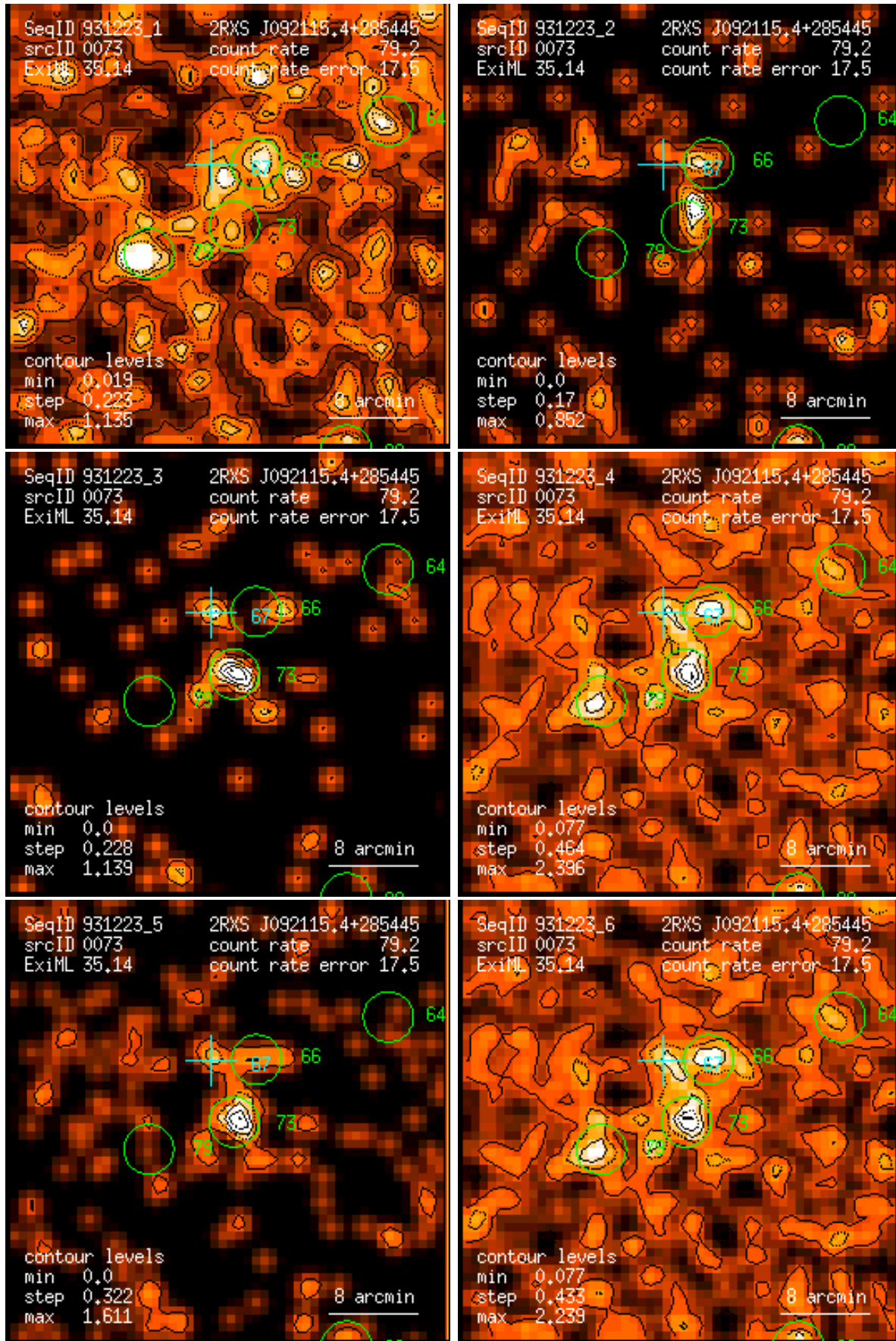
Figure 73: RASS 931223: detection 0073: band rate images, Gaussian filter: (1) PSPC channels 11 – 41, (2) 52 – 90, (3) 91 – 201, (4) 11 – 235, (5) 52 – 201, (6) 11 – 201. Broad band rates in counts/ks. Band rate contour levels in counts/ks/arcmin 2 .
