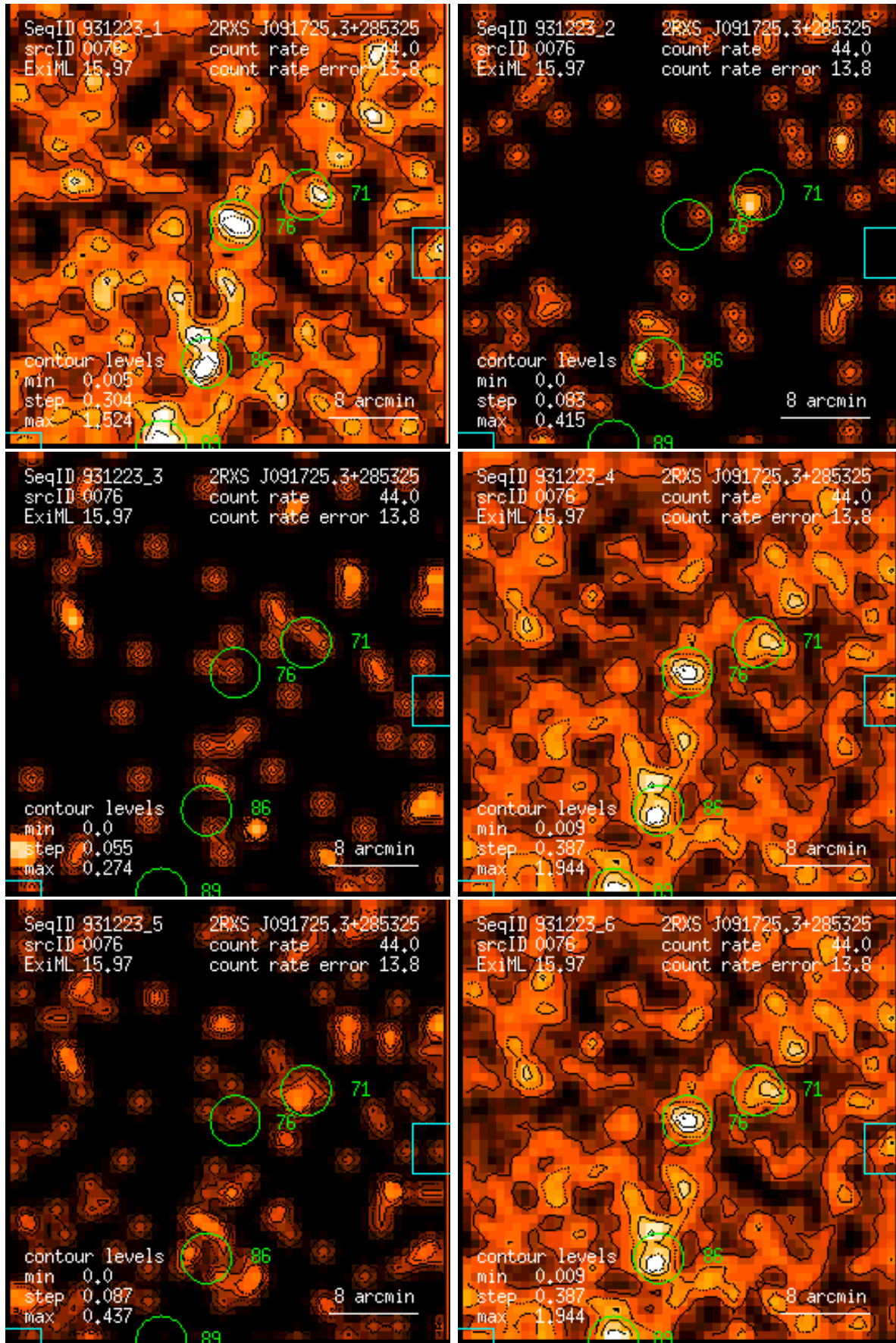
Figure 76: RASS 931223: detection 0076: band rate images, Gaussian filter: (1) PSPC channels 11 – 41, (2) 52 – 90, (3) 91 – 201, (4) 11 – 235, (5) 52 – 201, (6) 11 – 201. Broad band rates in counts/ks. Band rate contour levels in counts/ks/arcmin 2 .
