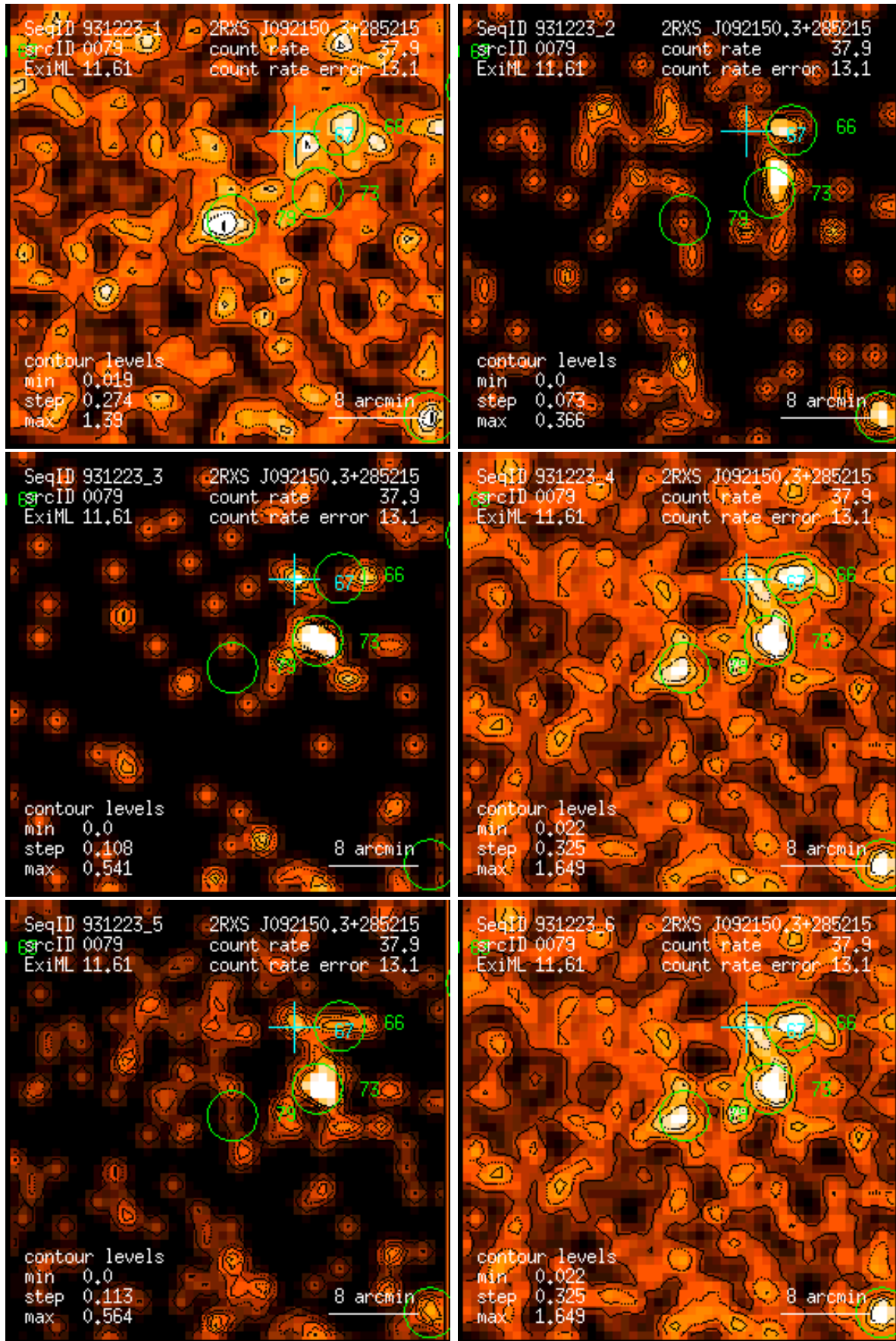
Figure 79: RASS 931223: detection 0079: band rate images, Gaussian filter: (1) PSPC channels 11 – 41, (2) 52 – 90, (3) 91 – 201, (4) 11 – 235, (5) 52 – 201, (6) 11 – 201. Broad band rates in counts/ks. Band rate contour levels in counts/ks/arcmin 2 .
