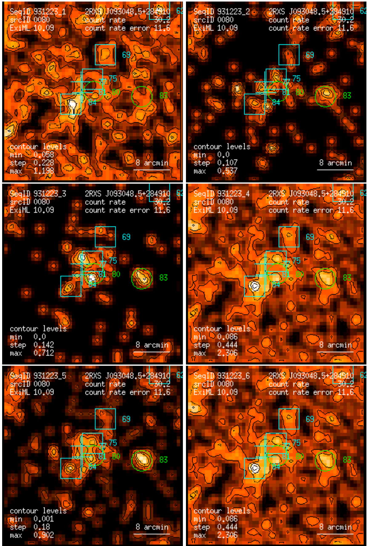
Figure 80: RASS 931223: detection 0080: band rate images, Gaussian filter: (1) PSPC channels 11 – 41, (2) 52 – 90, (3) 91 – 201, (4) 11 – 235, (5) 52 – 201, (6) 11 – 201. Broad band rates in counts/ks. Band rate contour levels in counts/ks/arcmin 2 .
