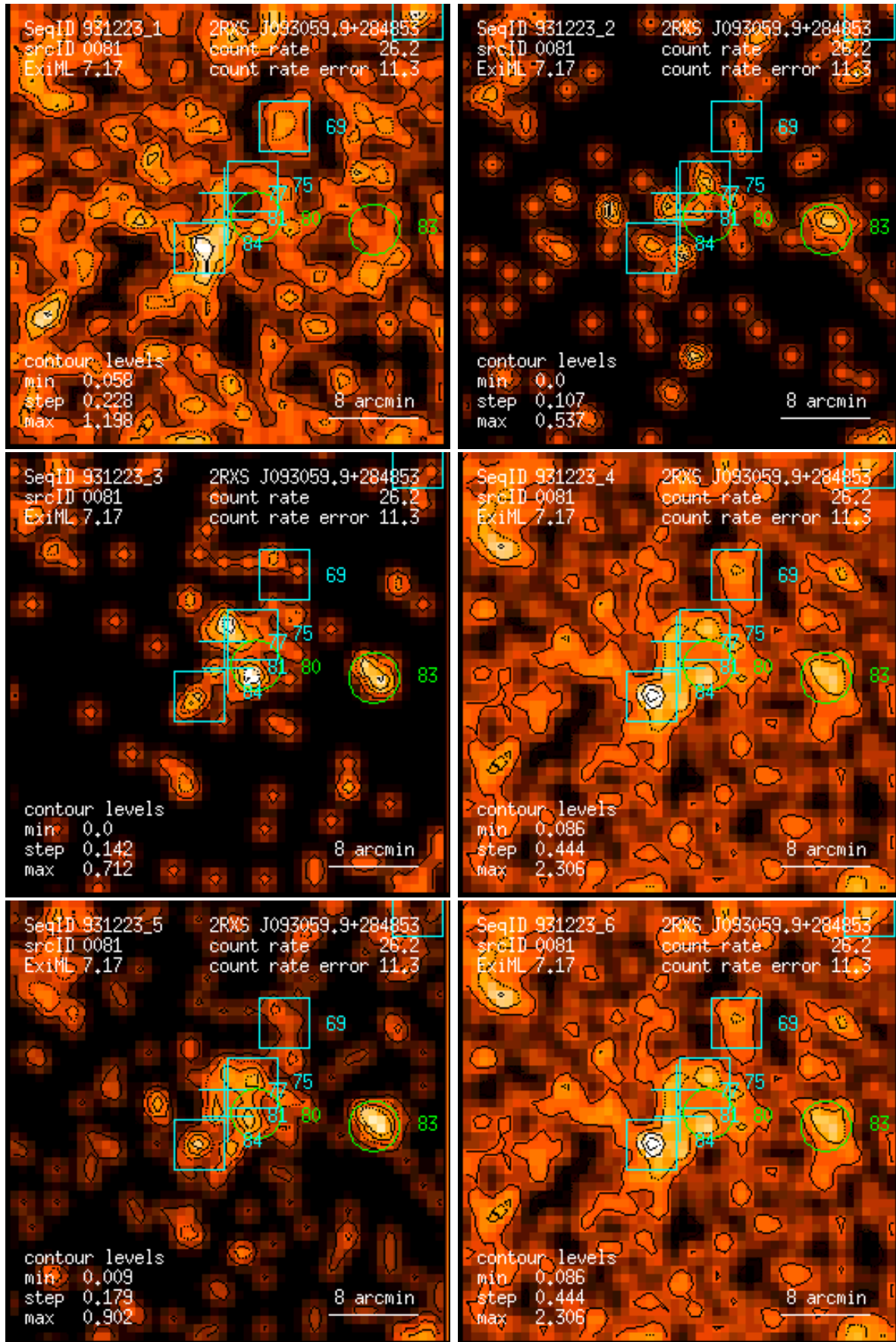
Figure 81: RASS 931223: detection 0081: band rate images, Gaussian filter: (1) PSPC channels 11 – 41, (2) 52 – 90, (3) 91 – 201, (4) 11 – 235, (5) 52 – 201, (6) 11 – 201. Broad band rates in counts/ks. Band rate contour levels in counts/ks/arcmin 2 .
