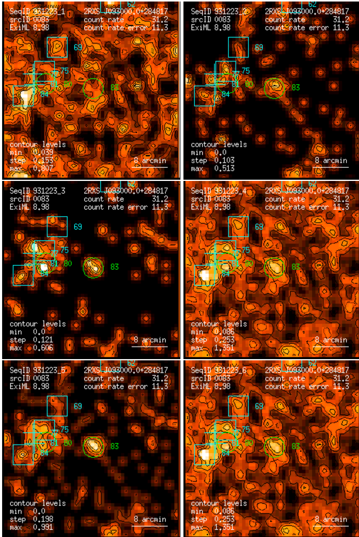
Figure 83: RASS 931223: detection 0083: band rate images, Gaussian filter: (1) PSPC channels 11 – 41, (2) 52 – 90, (3) 91 – 201, (4) 11 – 235, (5) 52 – 201, (6) 11 – 201. Broad band rates in counts/ks. Band rate contour levels in counts/ks/arcmin 2 .
