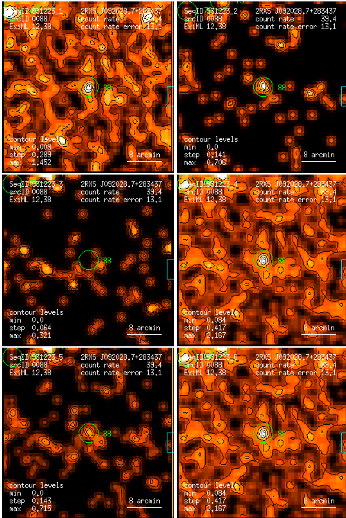
Figure 88: RASS 931223: detection 0088: band rate images, Gaussian filter: (1) PSPC channels 11 – 41, (2) 52 – 90, (3) 91 – 201, (4) 11 – 235, (5) 52 – 201, (6) 11 – 201. Broad band rates in counts/ks. Band rate contour levels in counts/ks/arcmin 2 .
