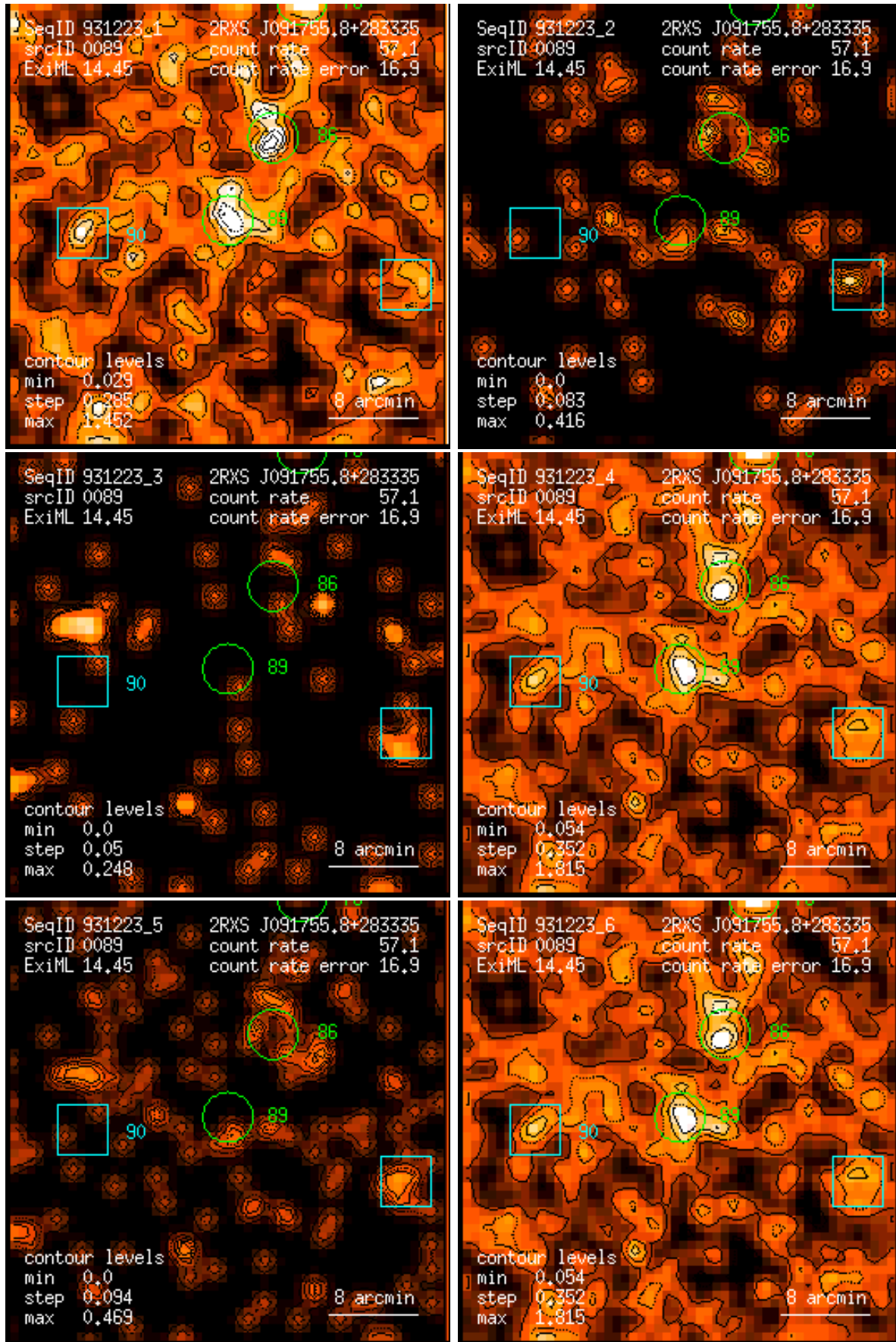
Figure 89: RASS 931223: detection 0089: band rate images, Gaussian filter: (1) PSPC channels 11 – 41, (2) 52 – 90, (3) 91 – 201, (4) 11 – 235, (5) 52 – 201, (6) 11 – 201. Broad band rates in counts/ks. Band rate contour levels in counts/ks/arcmin 2 .
