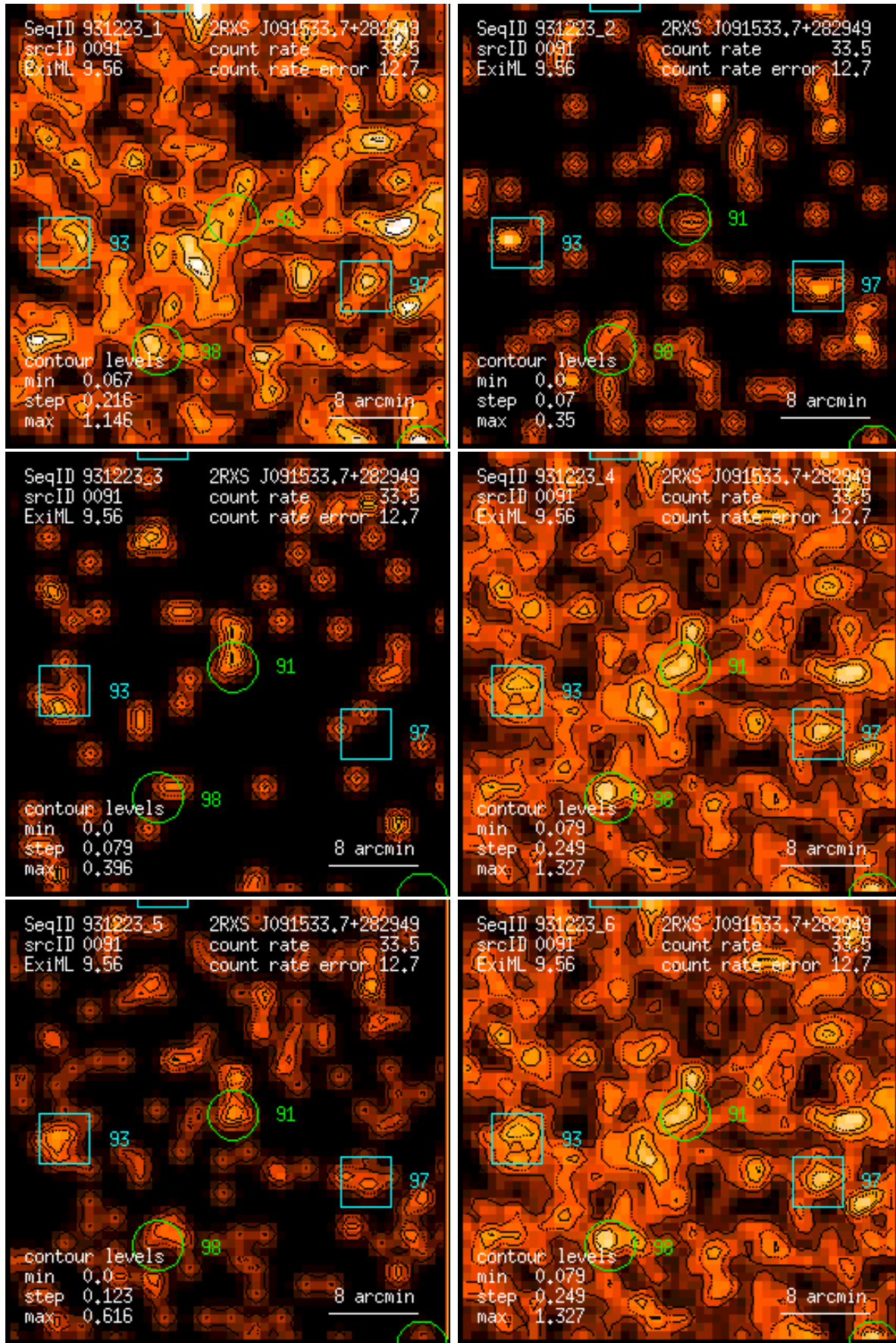
Figure 91: RASS 931223: detection 0091: band rate images, Gaussian filter: (1) PSPC channels 11 – 41, (2) 52 – 90, (3) 91 – 201, (4) 11 – 235, (5) 52 – 201, (6) 11 – 201. Broad band rates in counts/ks. Band rate contour levels in counts/ks/arcmin 2 .
