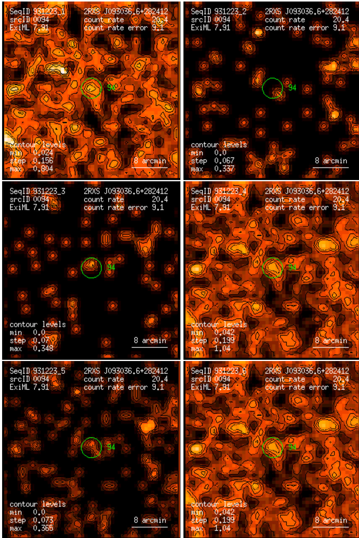
Figure 94: RASS 931223: detection 0094: band rate images, Gaussian filter: (1) PSPC channels 11 – 41, (2) 52 – 90, (3) 91 – 201, (4) 11 – 235, (5) 52 – 201, (6) 11 – 201. Broad band rates in counts/ks. Band rate contour levels in counts/ks/arcmin 2 .
