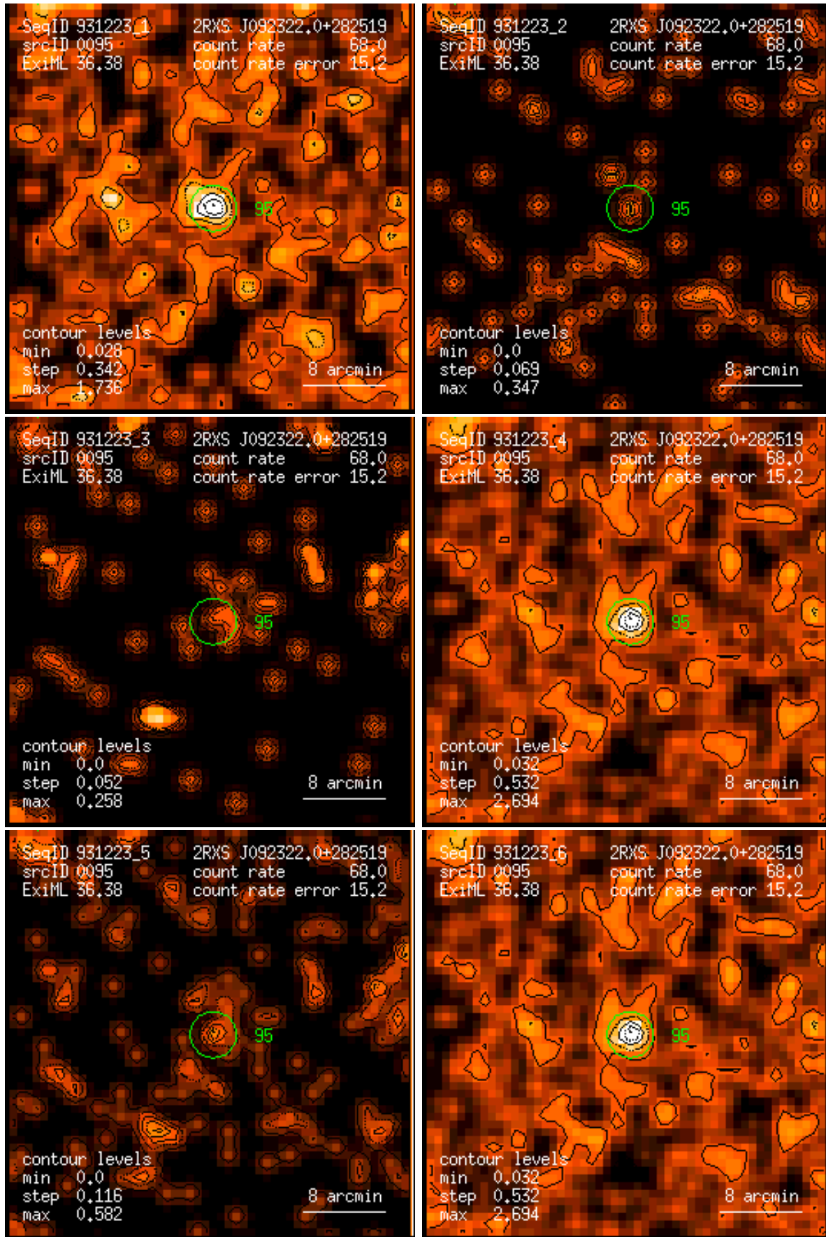
Figure 95: RASS 931223: detection 0095: band rate images, Gaussian filter: (1) PSPC channels 11 – 41, (2) 52 – 90, (3) 91 – 201, (4) 11 – 235, (5) 52 – 201, (6) 11 – 201. Broad band rates in counts/ks. Band rate contour levels in counts/ks/arcmin 2 .
