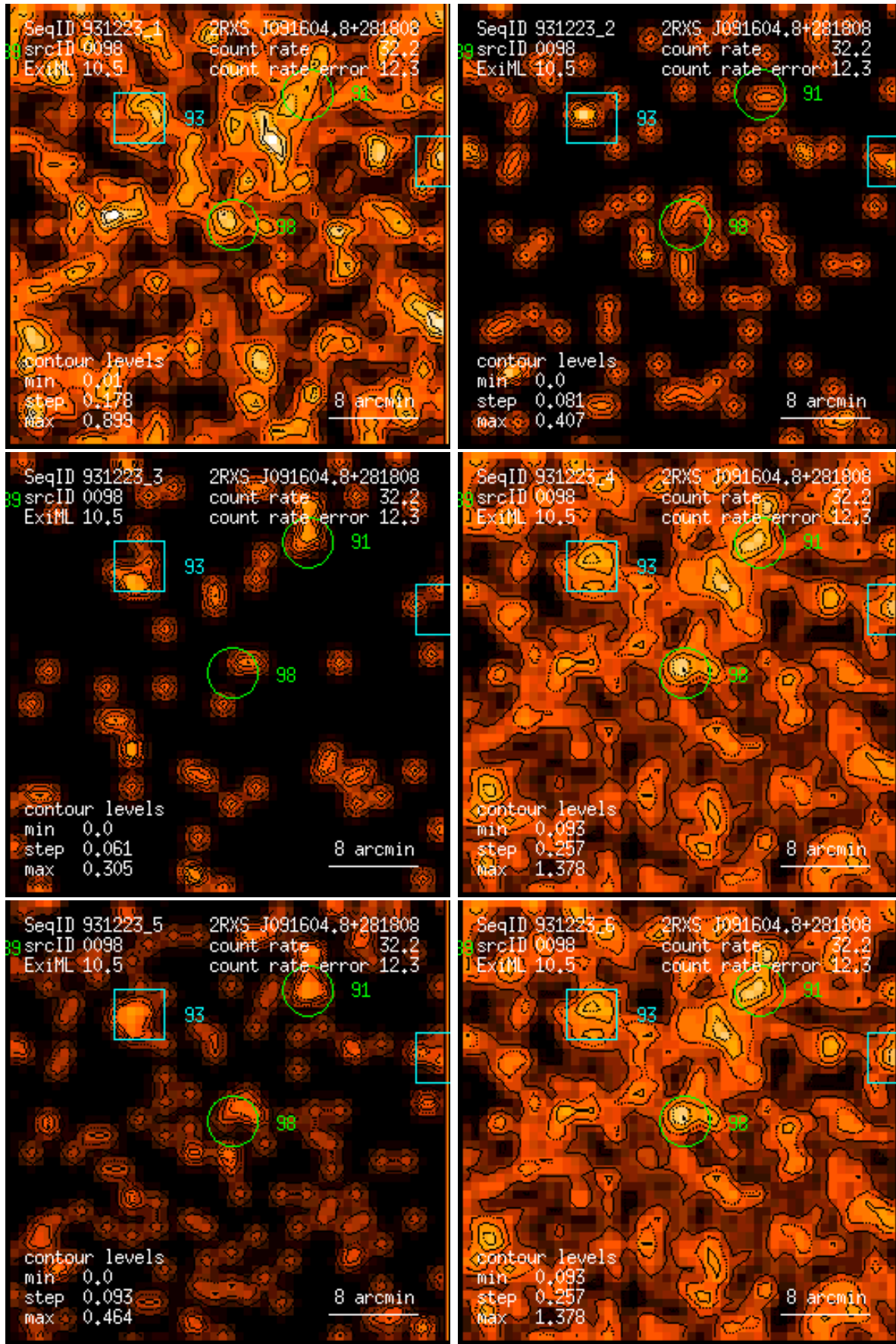
Figure 98: RASS 931223: detection 0098: band rate images, Gaussian filter: (1) PSPC channels 11 – 41, (2) 52 – 90, (3) 91 – 201, (4) 11 – 235, (5) 52 – 201, (6) 11 – 201. Broad band rates in counts/ks. Band rate contour levels in counts/ks/arcmin 2 .
