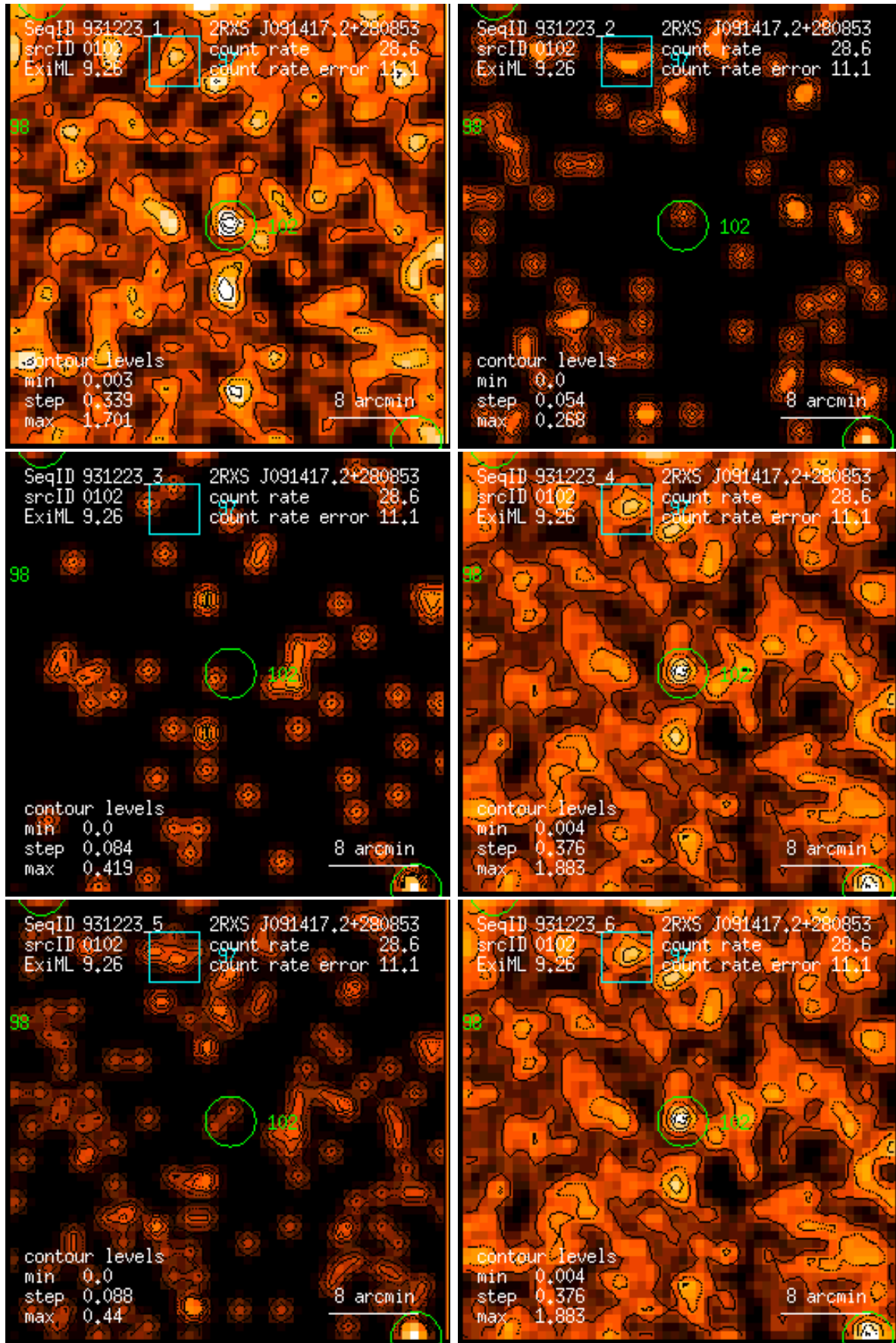
Figure 102: RASS 931223: detection 0102: band rate images, Gaussian filter: (1) PSPC channels 11 – 41, (2) 52 – 90, (3) 91 – 201, (4) 11 – 235, (5) 52 – 201, (6) 11 – 201. Broad band rates in counts/ks. Band rate contour levels in counts/ks/arcmin 2 .
